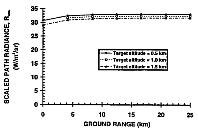
Figure 8 Scale Parameters for the Mid-Latitude Summer Case
