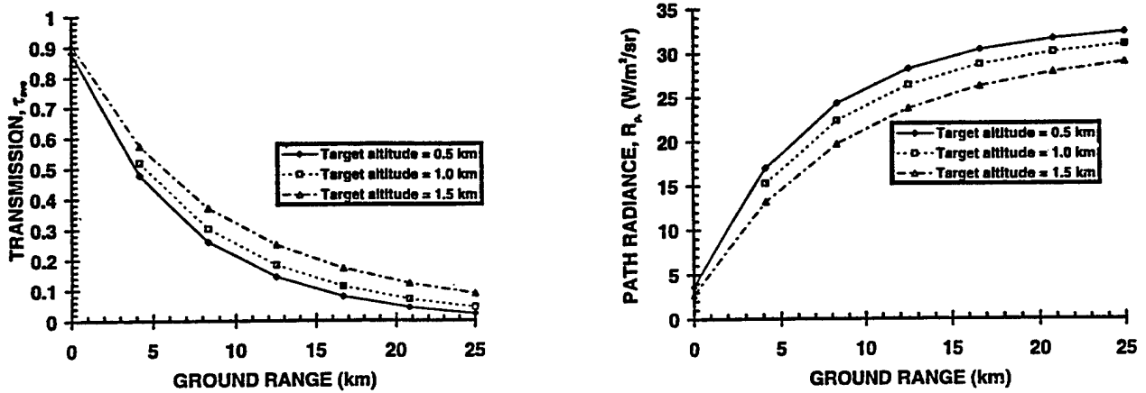
Figure 6 Path Transmission and Radiance for the Mid-Latitude Summer Case
