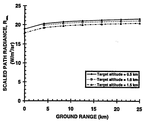
Figure 7 Scale Parameters for the Mid-Latitude Winter Case
