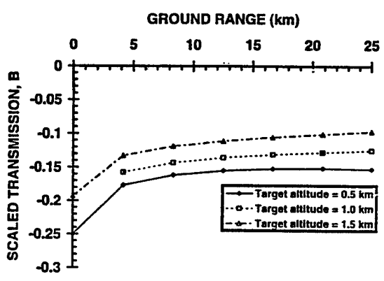
Figure 7 Scale Parameters for the Mid-Latitude Winter Case
