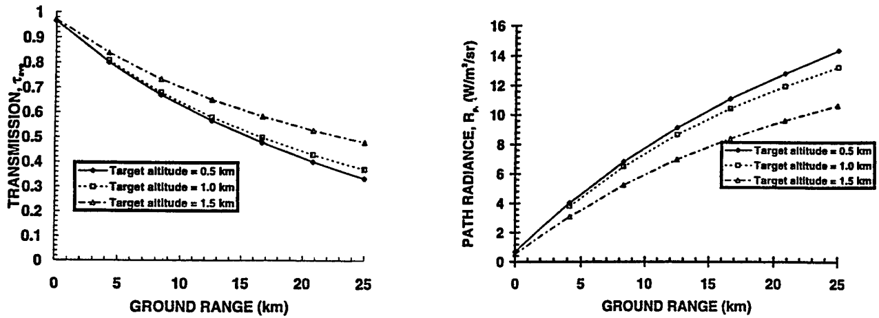
Figure 5 Path Transmission and Radiance for the Mid-Latitude Winter Case
