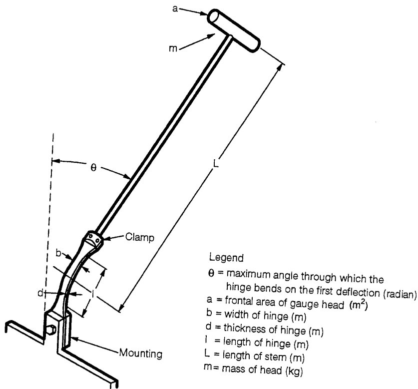
Figure 3. DPI Gauge
