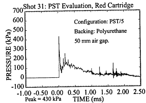
Figure 5 (continued) - Pressure-time profiles from the portable shock tube for shots 25 to 32.
