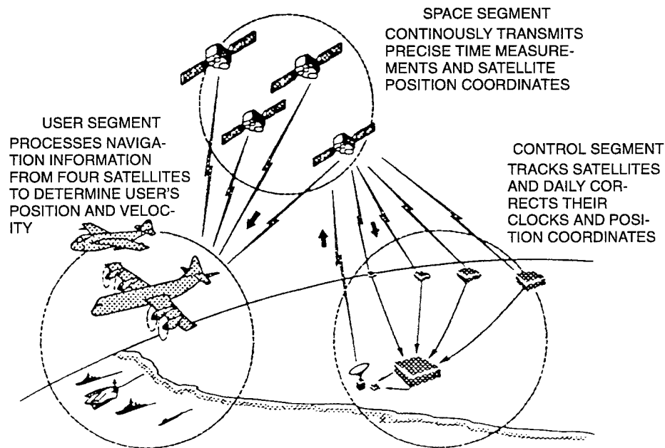
NAVSTAR GPS program segments.
