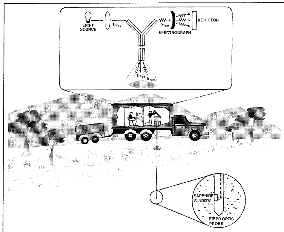
Cone Penetrometer Fiber-Optic Fluorometer (Double Fiber System).
