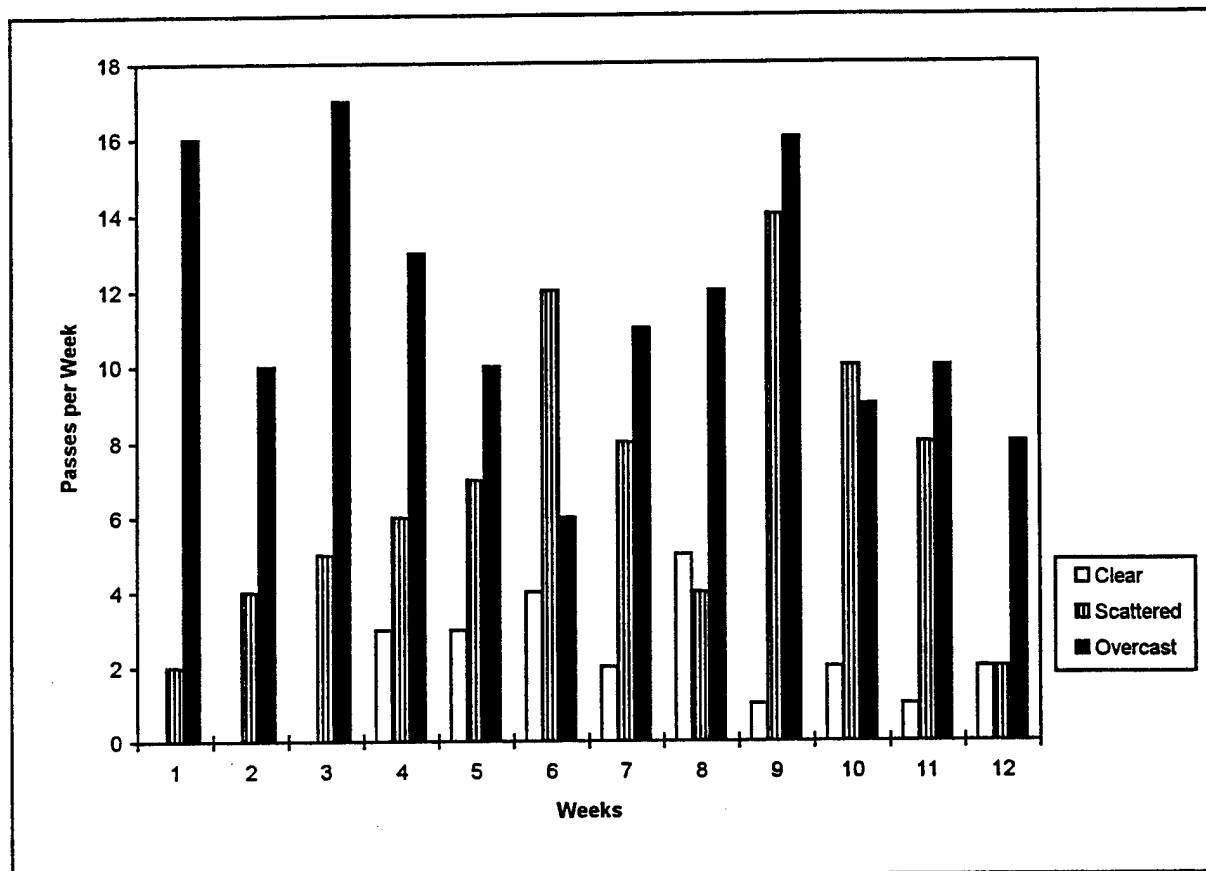
Figure 10. Total number of clear, scattered clouds, and cloudy images collected per week during the 1993 DCC Experiment.
