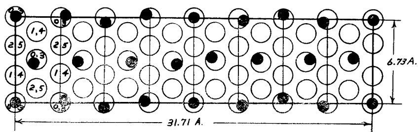
Fig. 8--Projection of the U_2O_5 structure on (001)--C arrangement. (The solid circles are uranium atoms; the open circles are oxygen atoms as in UO_3 . The numbers refer to the z coordinates in sixths.)
