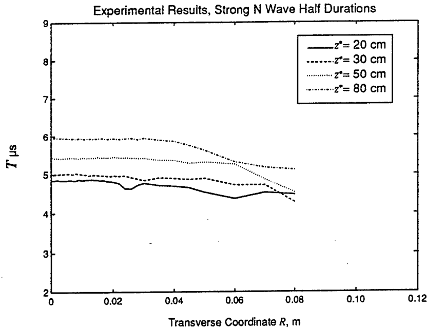
Figure 2.3 Measured half duration T as a function of R at various axial distances
