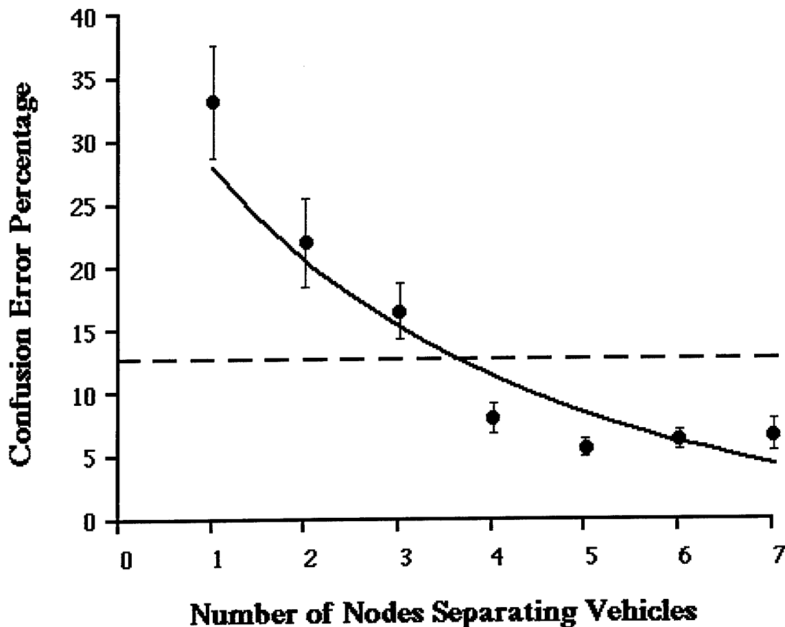
Figure 3. Nodal Distance chart
