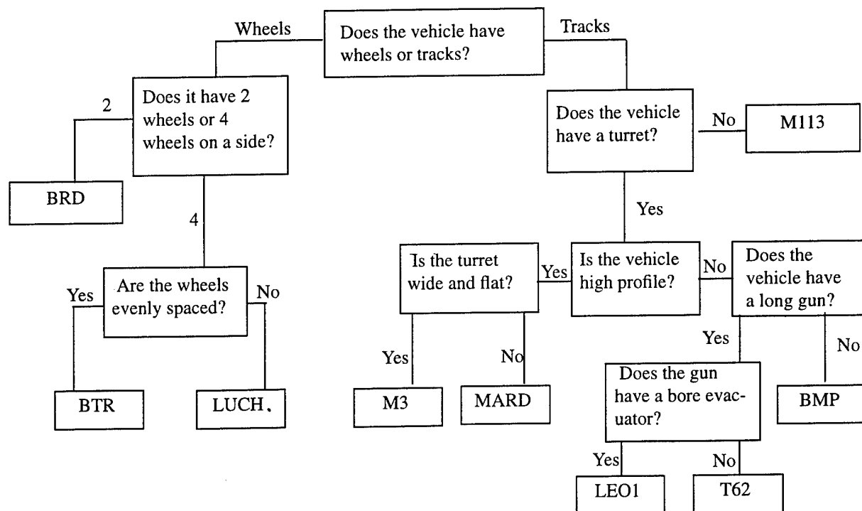
Figure 2. Similarity Decision Tree
