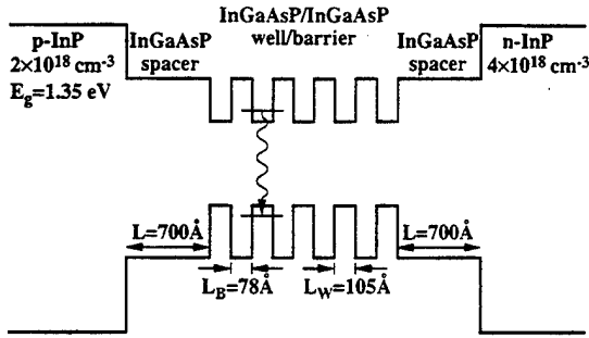
Fig. 2. The conduction and valence band edge profiles for the InGaAsP strained quantum-well laser under study. The InGaAsP well region is slightly tensile strained with a PL wavelength of 1.485 \mu\text{m} . The barrier InGaAsP regions are lattice-matched to InP and its bandgap wavelength is 1.28 \mu\text{m} .
