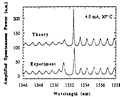
CMF6 Fig. 1 A plot of the amplified spontaneous emission spectrum taken at 30°C with an injection current of 4 mA ( I_m = 4.7 mA). Theory is shown offset from the experimental data.
