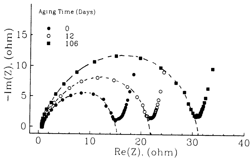
Figure 35. Impedance spectra of the Li_{1.0}Mn_2O_{4.7} cathode in the Li//SPE//Li_{1.0}Mn_2O_{4.7} Cell BMX29 relative to the Li reference taken at the beginning, 12 days and 106 days of storage at 25^\circ C
