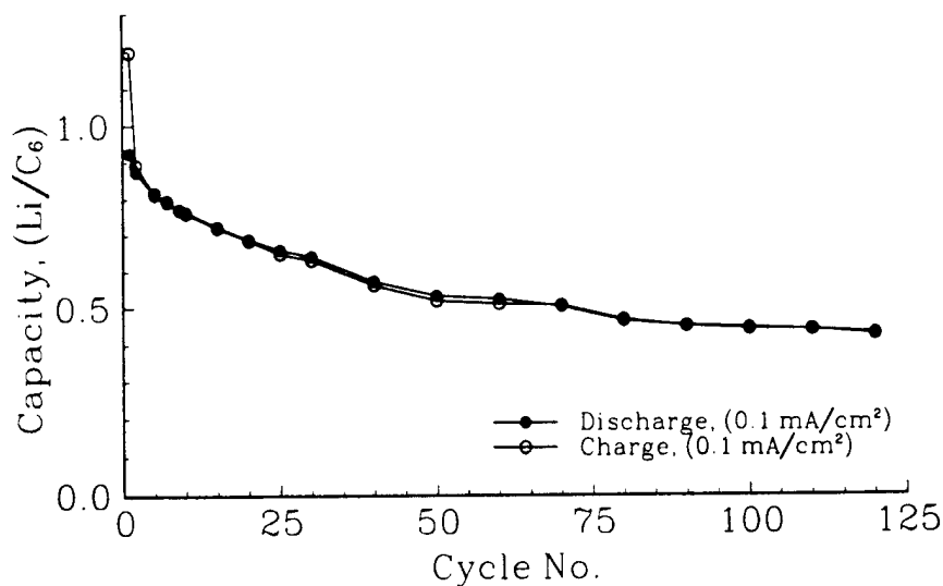
Figure 57. Capacity versus cycles for the cell shown in Figure 56.
