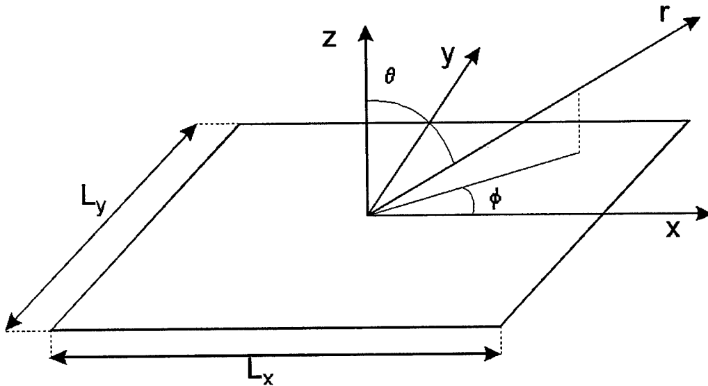
Figure 2. Coordinate System for Scattering from a Planar Rectangular Plate
