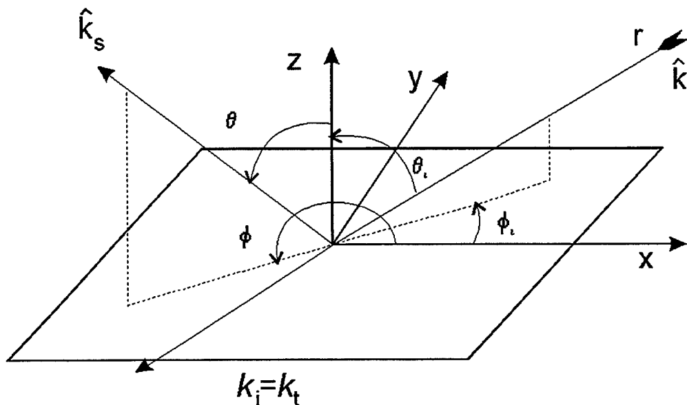
Figure 1. Reflection and Transmission from a Resistive Sheet
