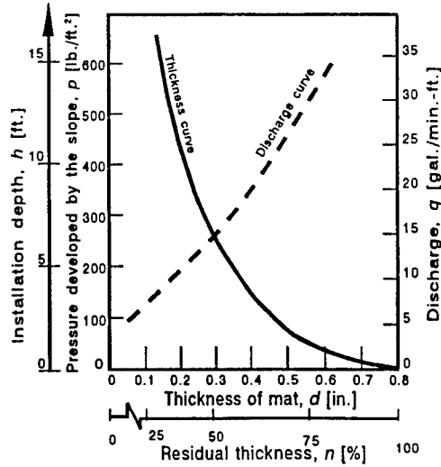
(b) Enkadrain at a hydraulic gradient of 1.0
