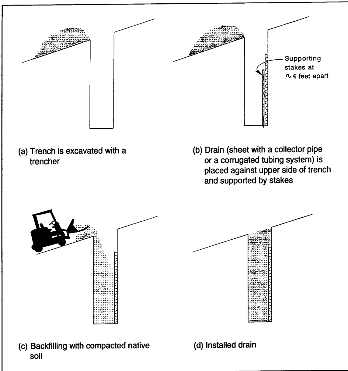
Figure 20. Construction scheme
