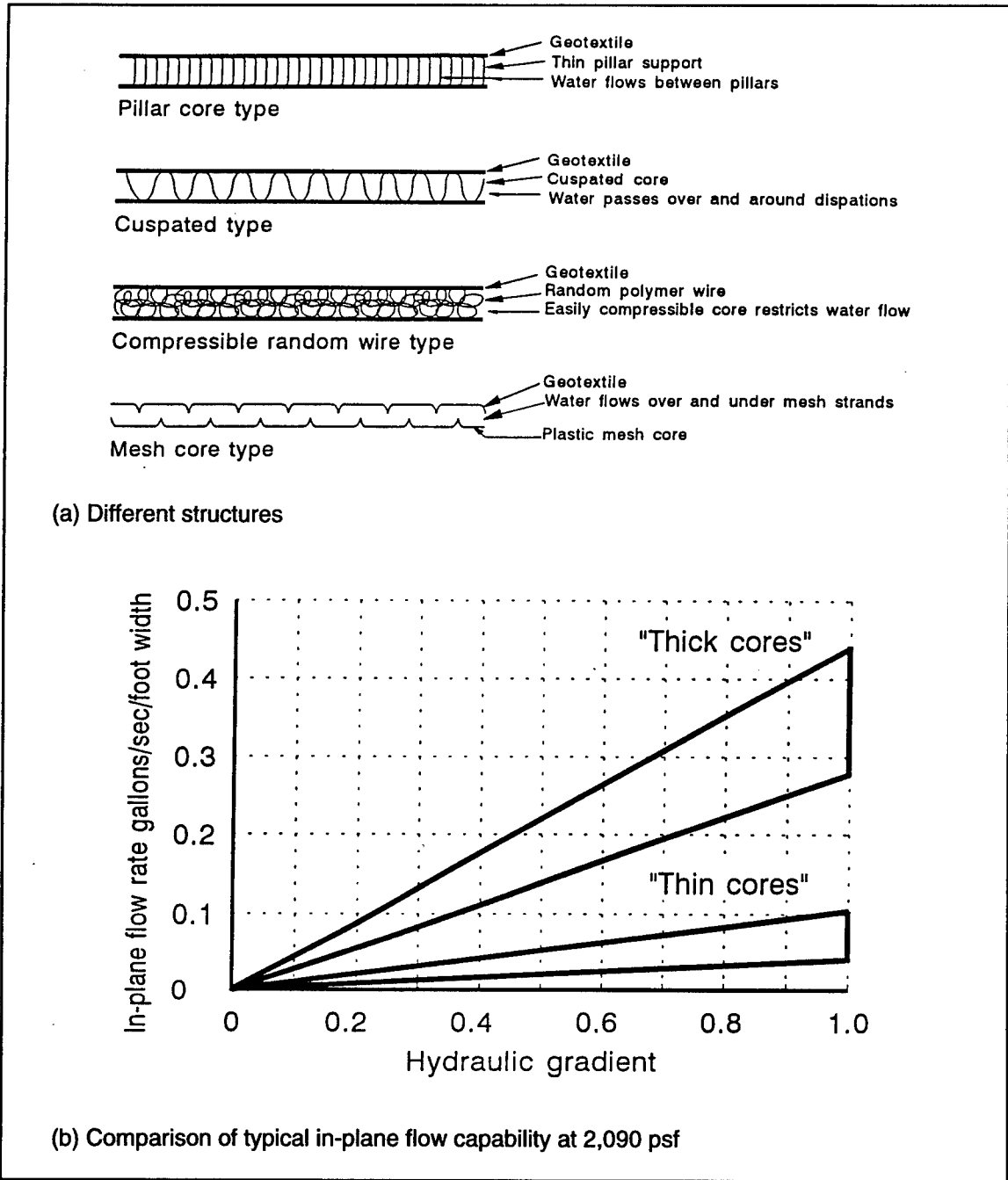
Figure 4. Flow capabilities of geocomposite drains (after Murray and McGown 1992)
