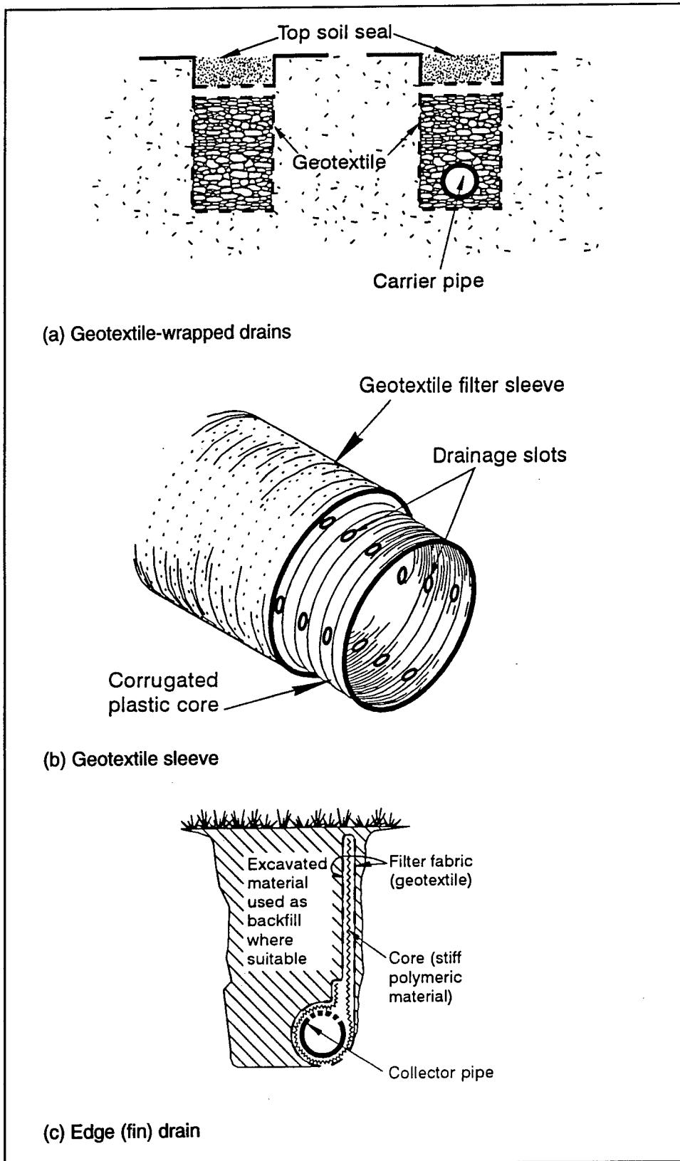
Figure 1. Typical geocomposite drainage systems (after Murray and McGown 1992)
