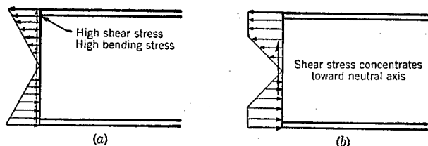
FIG. 4.—BENDING AND SHEAR
