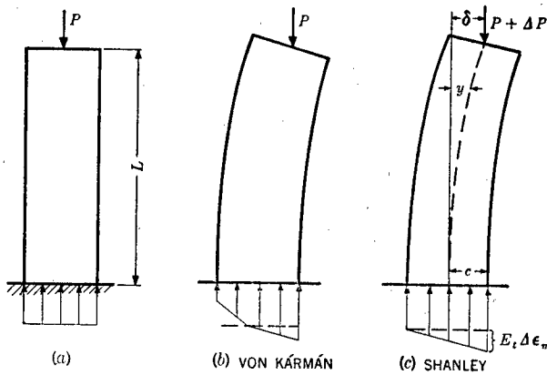
FIG. 6.—COLUMN INSTABILITY (PLASTIC)
