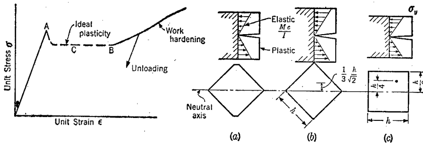
FIG. 1.—STRESS-STRAIN DIAGRAM FOR STRUCTURAL STEEL
