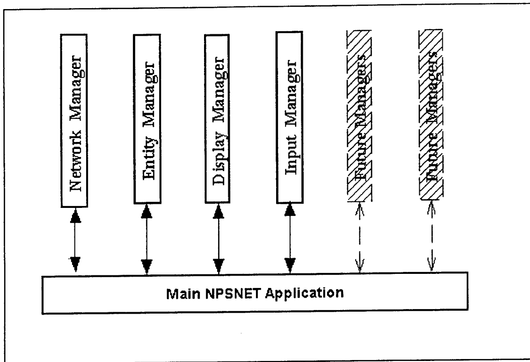
Figure 12: Proposed NPSNET Architecture [BARK96]
