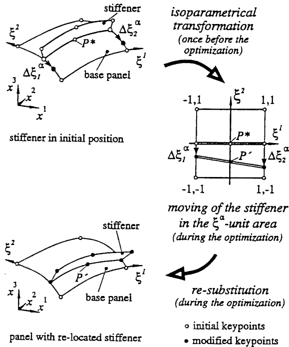
Fig. 14: Moving of a stiffener using design elements
