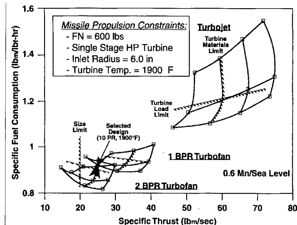
Figure 5 - Uninstalled Performance Trades (With Constraints)
