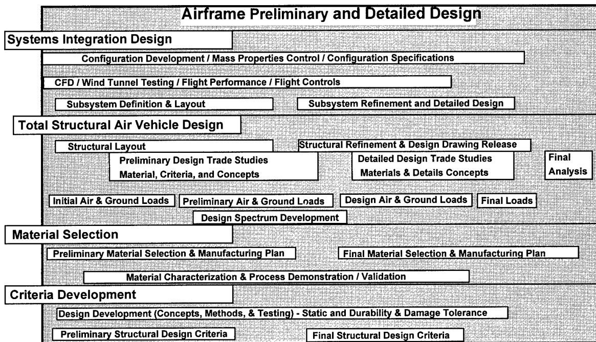
Figure 2 Many Processes Integrated Concurrently For Structural Certification
