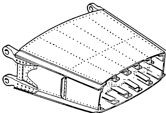
Fig. 1: Torsion box typical configuration
