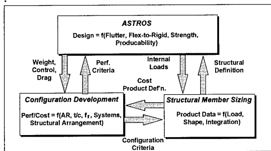
Figure 5 ASTROS In The Internal Loads Process
