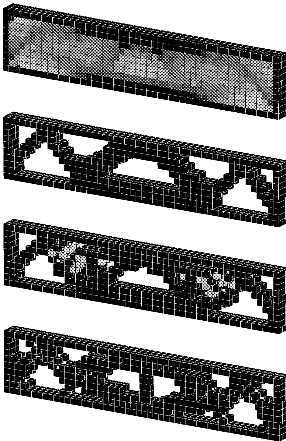
Figure 5 - Volume Fraction Distribution for 3D beam ( \mu \geq 0.1 ). Top to Bottom cases 1 to 4.
