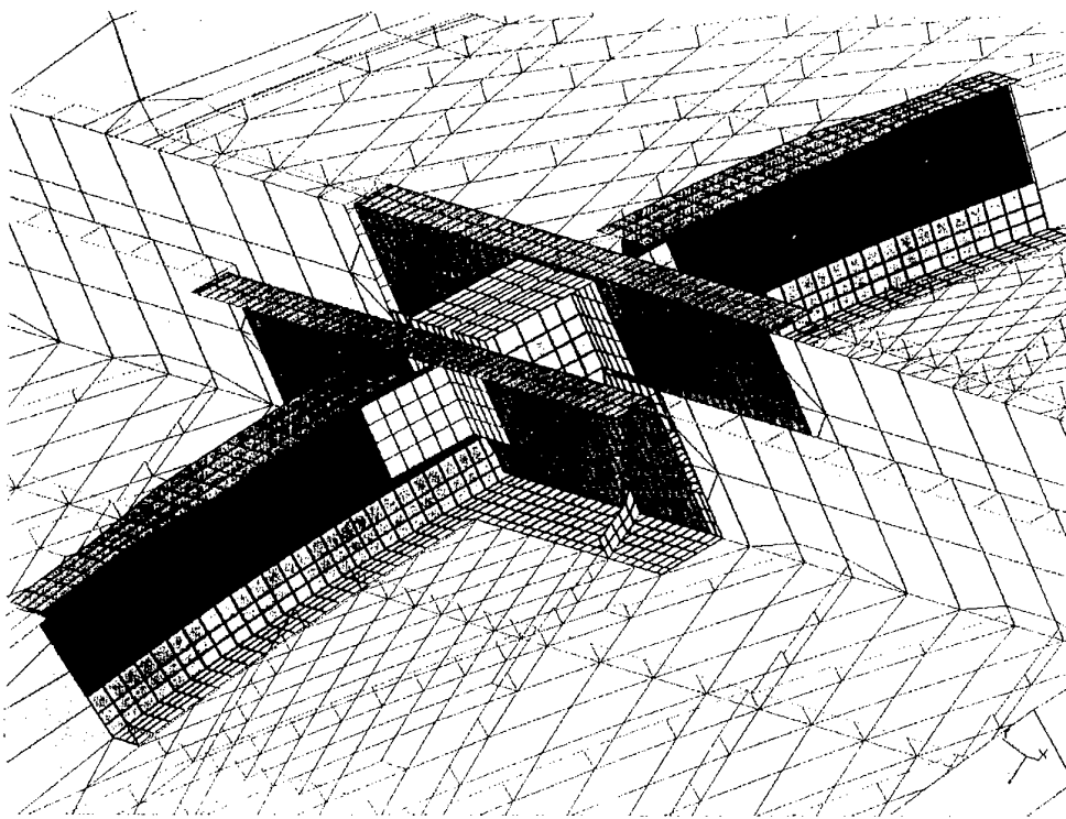
Fig. 8 Ring/Longeron Connection
