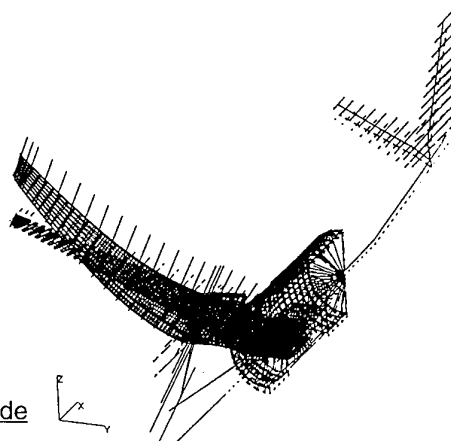
Fig. 16: comparison of mode shapes calculated with the simple beam model and the complete FE-model.
