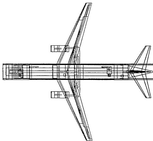
Fig. 8: electronic mass-distribution representation of the FA-X aircraft. The model contains approximately 250 mass-items.
