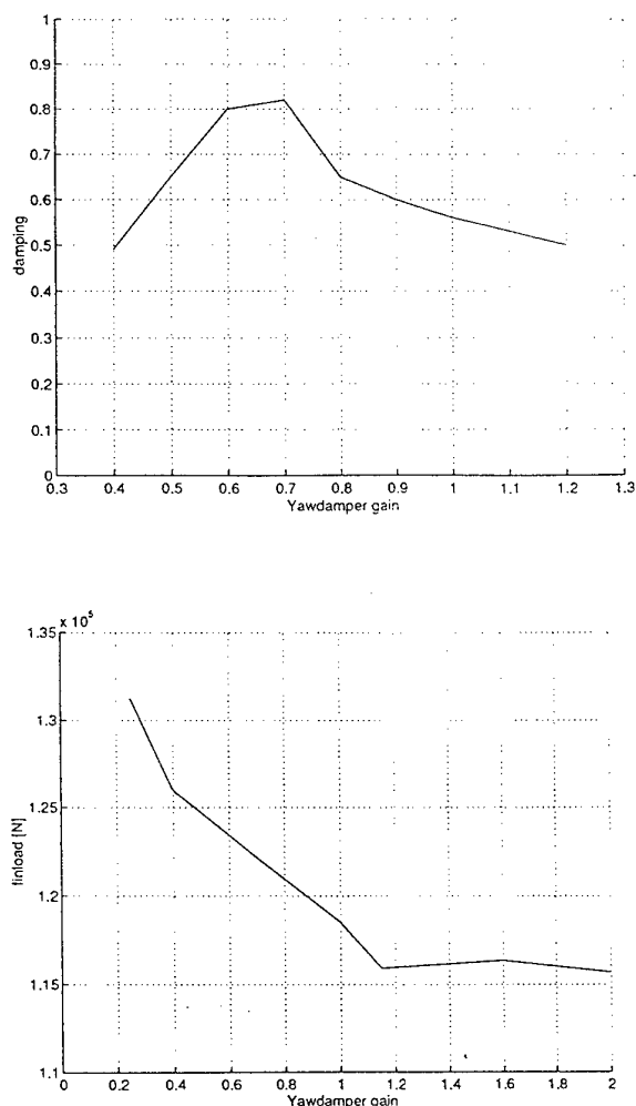
Fig. 13: damping and fin loads as a function of yaw damper gain .
