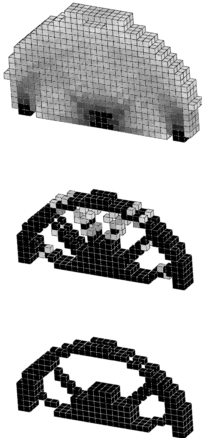
Figure 7 - Volume Fraction Distribution for bicycle wheel ( \mu\zeta 0.1 ). Top to Bottom cases 1 to 3.
