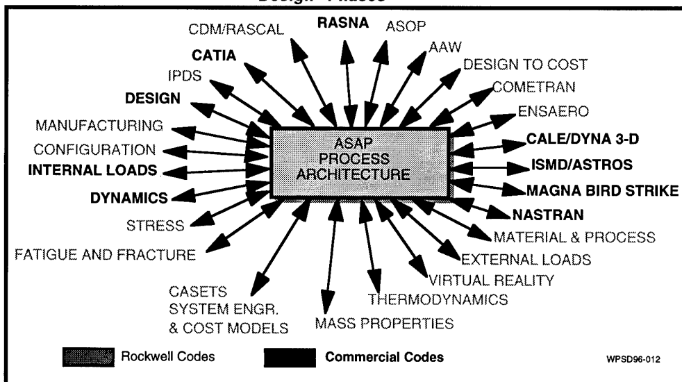
Figure 8. The Automated Structural Analysis Process (ASAP)
