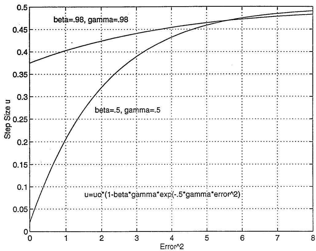
Figure 6a Variation of u with \text{Error}^2 for u_0 = .05
