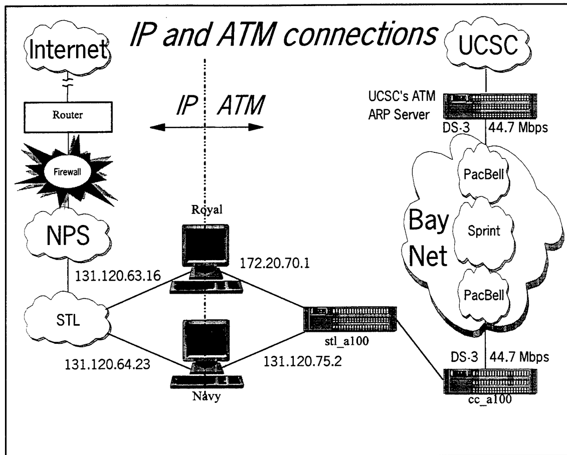
Figure 19. NPS ATM LAN — IP and ATM connections.
