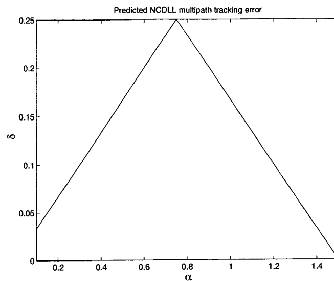
Figure 12. Predicted NCDLL multipath tracking error for a_0 = 1 , a_1 = 0.5 , and \theta_0 - \theta_1 = 2n\pi (for n an integer).
