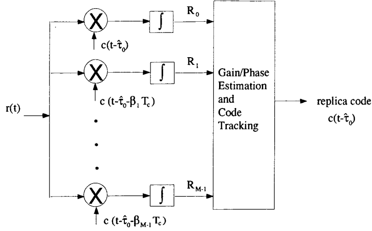
Figure 5. Multiple-correlator estimation.
