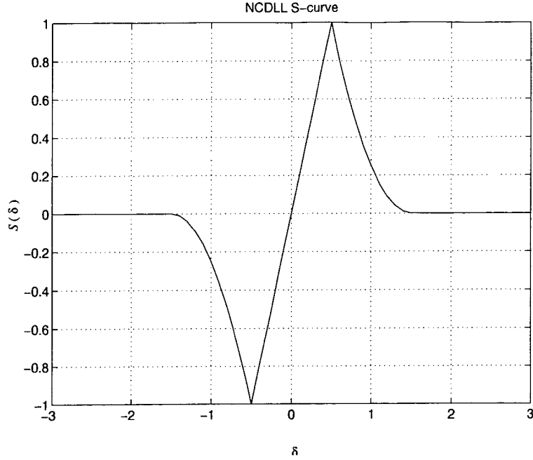
Figure 7. NCDLL S-curve.
