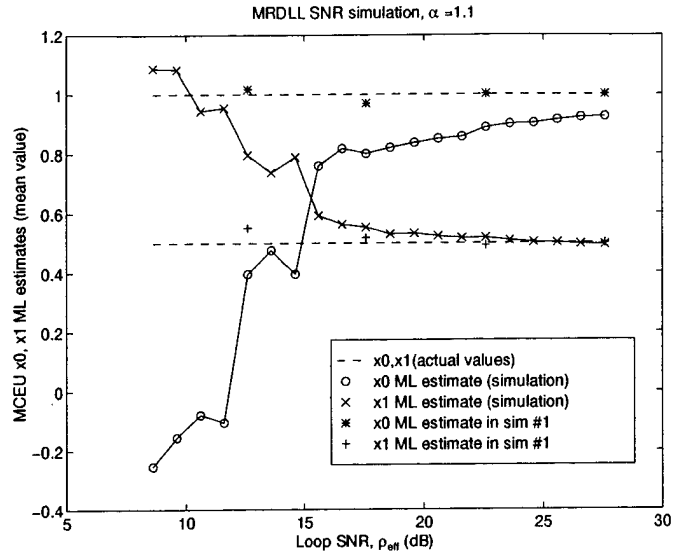
Figure 75. Simulation results showing MCEU ML estimate, \hat{\mathbf{x}} for different values of effective MCTL loop SNR, \rho_{eff} (in dB) when \alpha = 1.1 .
