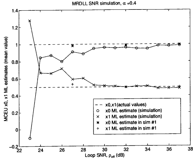
Figure 69. Simulation results showing MCEU ML estimate, \hat{\mathbf{x}} for different values of effective MCTL loop SNR, \rho_{eff} (in dB) when \alpha = 0.4 .
