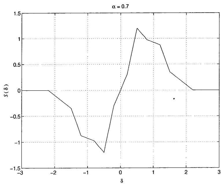
Figure 22. MRDLL S-curve with x_0 = 1 , x_1 = 0.5 , and \alpha = 0.7 .
