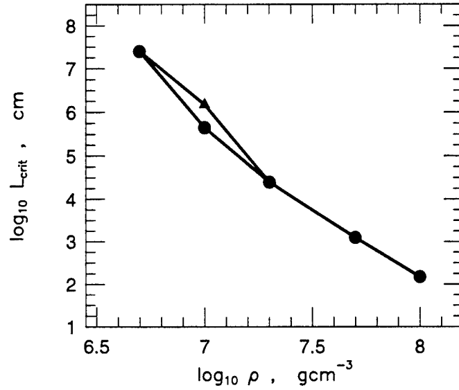
Fig. 6 - Critical length for the initiation of a detonation as a function of the fuel density. (Circles) - \Delta q = 4 \times 10^{17} ergs g -1 for deflagration products. (Triangles) - \Delta q = 3 \times 10^{17} ergs g -1 for deflagration products (all but one triangle coincide with the circles).
