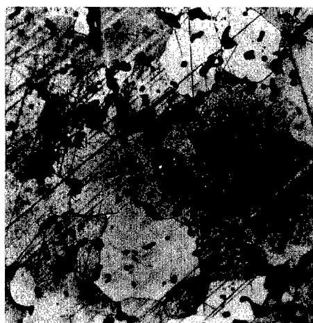
Fig. 22--Sintered Alloy, 4.1% Carbon, Heated at 2110^{\circ}\text{C} for 10 Minutes, Furnace-Cooled, Air-Etched, X 250.
