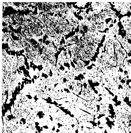
Fig. 16--Fused Sample, 0.6% Carbon, From Center of Thorium Billet Heated at 1870° to 1970°C for 20 Minutes in Contact With Graphite, Furnace-Cooled, Unetched, X 75.
