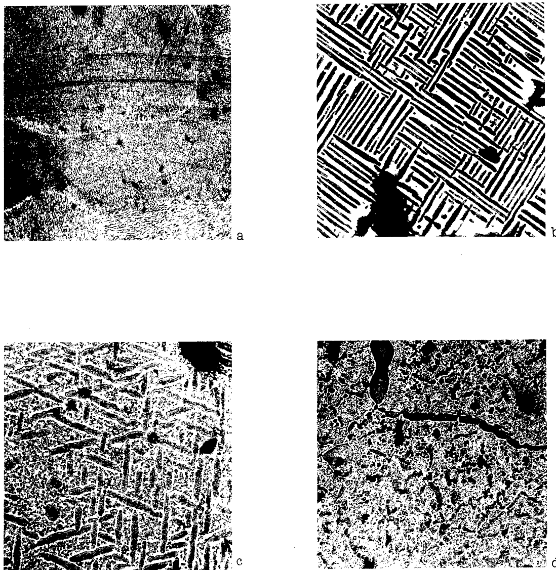
Fig. 37--Microstructures of a 1.5% Carbon Test Bar Annealed at 1690°C for 4.5 Hours and Then Rapidly Cooled in a Helium Atmosphere to Room Temperature. The Microstructure at the Upper Left is That of the Center of the Bar, and Figures from Left to Right Show Microstructures Taken Along the Bar Between the Midpoint and the Water-Cooled Copper Electrode at Points of Successively Decreasing Temperatures. Etched with 1 Nitric Acid - 2 Ethyl Alcohol - Sodium Fluosilicate Solution, X 250.
