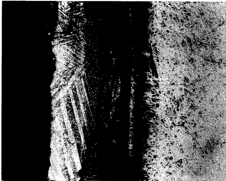
Fig. 13--Diffusion Bands of Carbide Formed by Heating Thorium in Contact With Graphite at 1860° to 1880°C for 30 Minutes, Oil-Quenched, Air-Etched, X 220
