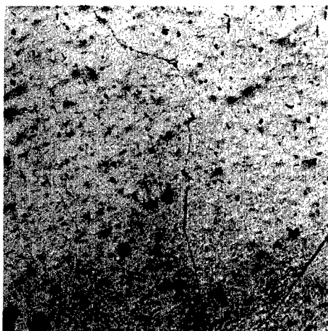
Fig. 15--Fused Sample, 0.3% Carbon, From Center of Thorium Billet Heated at 1770° to 1825°C for 19 Minutes in Contact With Graphite, Furnace-Cooled, Unetched, X 100.
