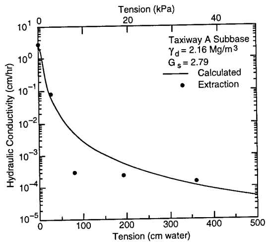
g. Taxiway A subbase.
