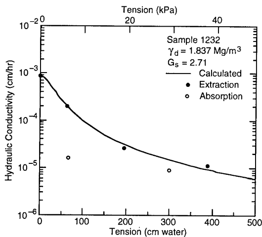
c. Subgrade sample 1232 (566).
