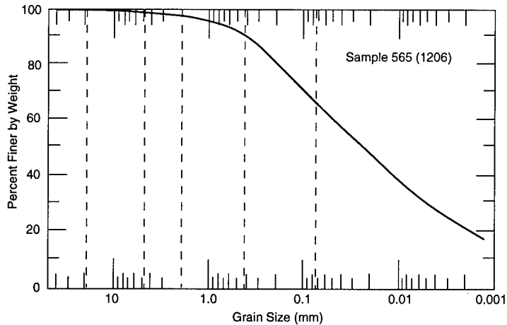
Figure 1. Grain size distribution of Mn/ROAD materials. Figures 1e to 1g that show the subbase and base materials include the range of Mn/DOT specifications.
