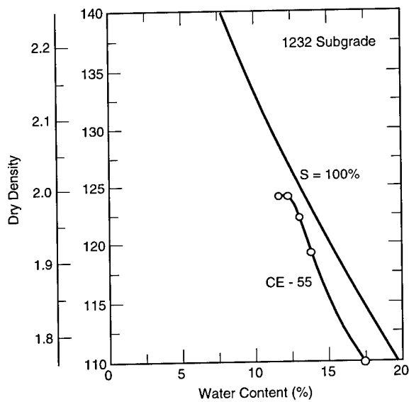
d. Subgrade sample 1232 (566).
