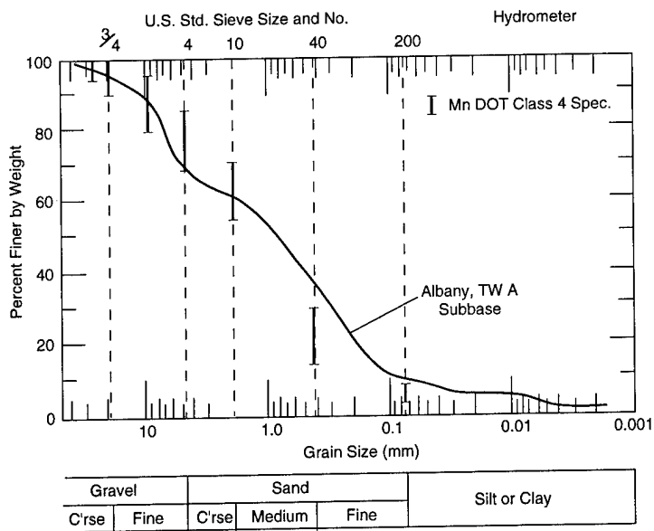
a. Albany taxiway A subbase/class 4 special base.
