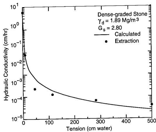
h. Dense-graded stone.
