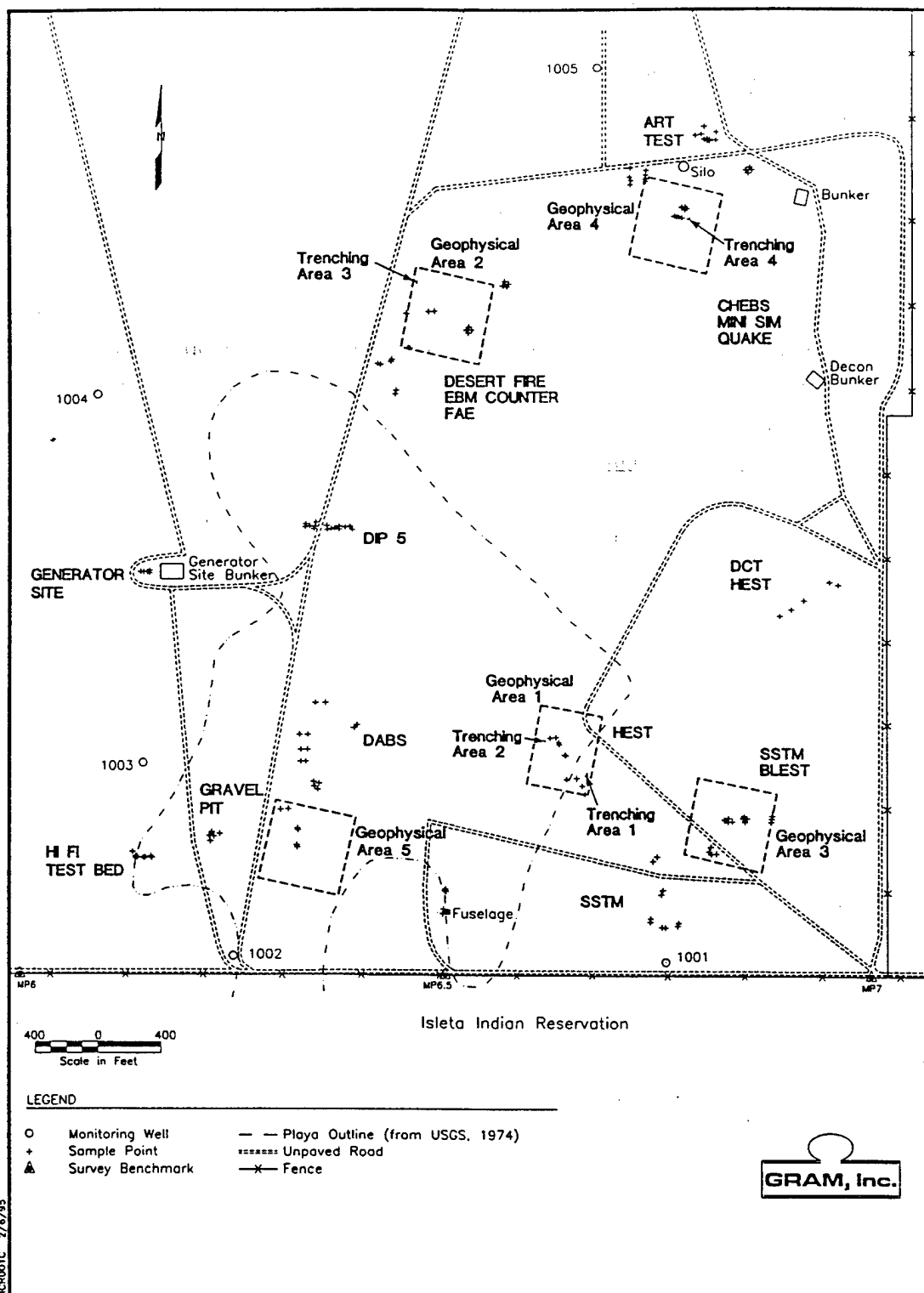
Figure 2.1 Locations Geophysical Surveys, Trenching Areas, and Hand-Auguring Areas
