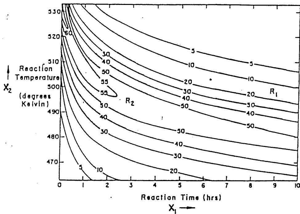
Fig. 10 Representative Response Surface Contour Plot
