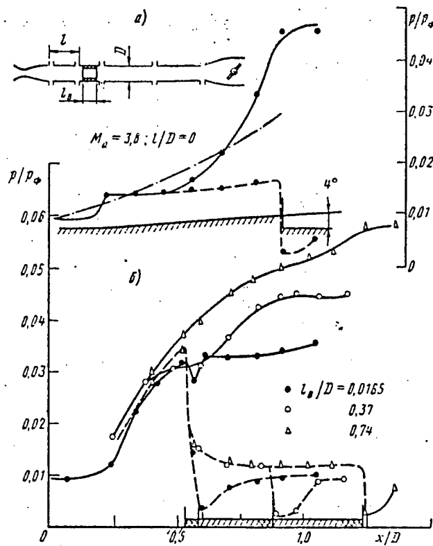
Fig. 3.3.1 Pressure distribution along obstacles.
