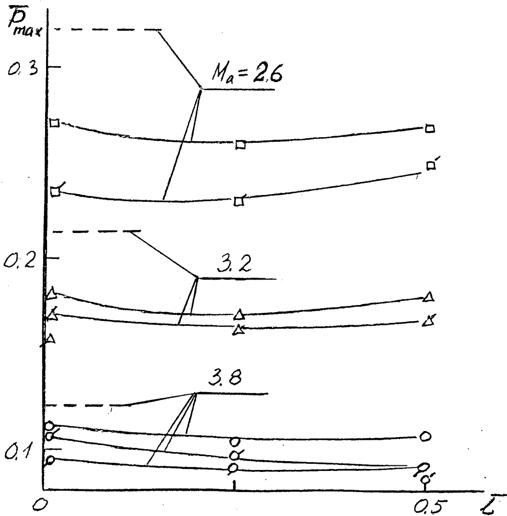
Fig. 3.1 12 P_{max} dependence on the grate width. Rhombic struts.
