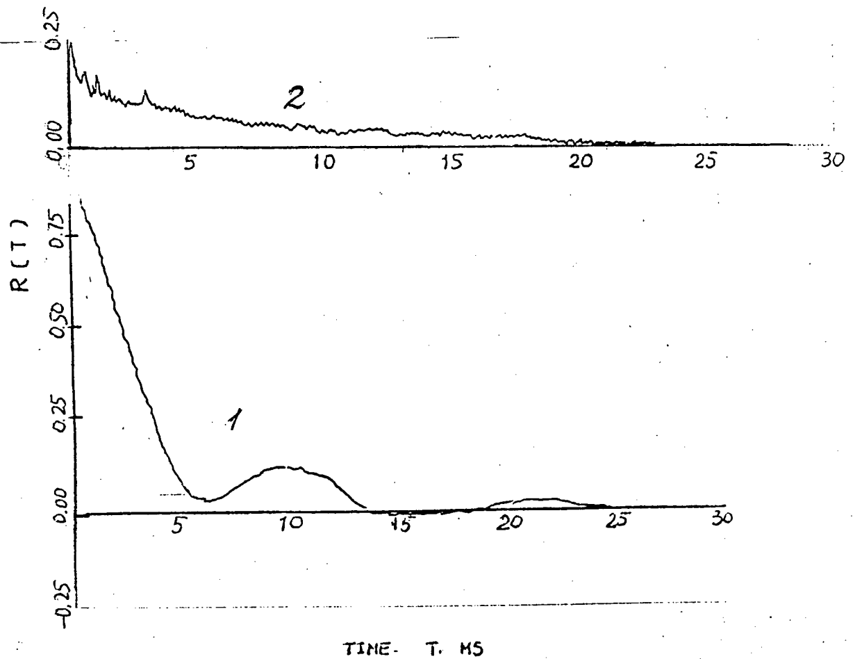
Fig 3.5.24 Power spectra density vs. frequency. Autocorrelation function vs. time. rhomb struts, — 1 row, Ma=3.2, pseudo-shock, r.3, static pressure pulsations, I section
