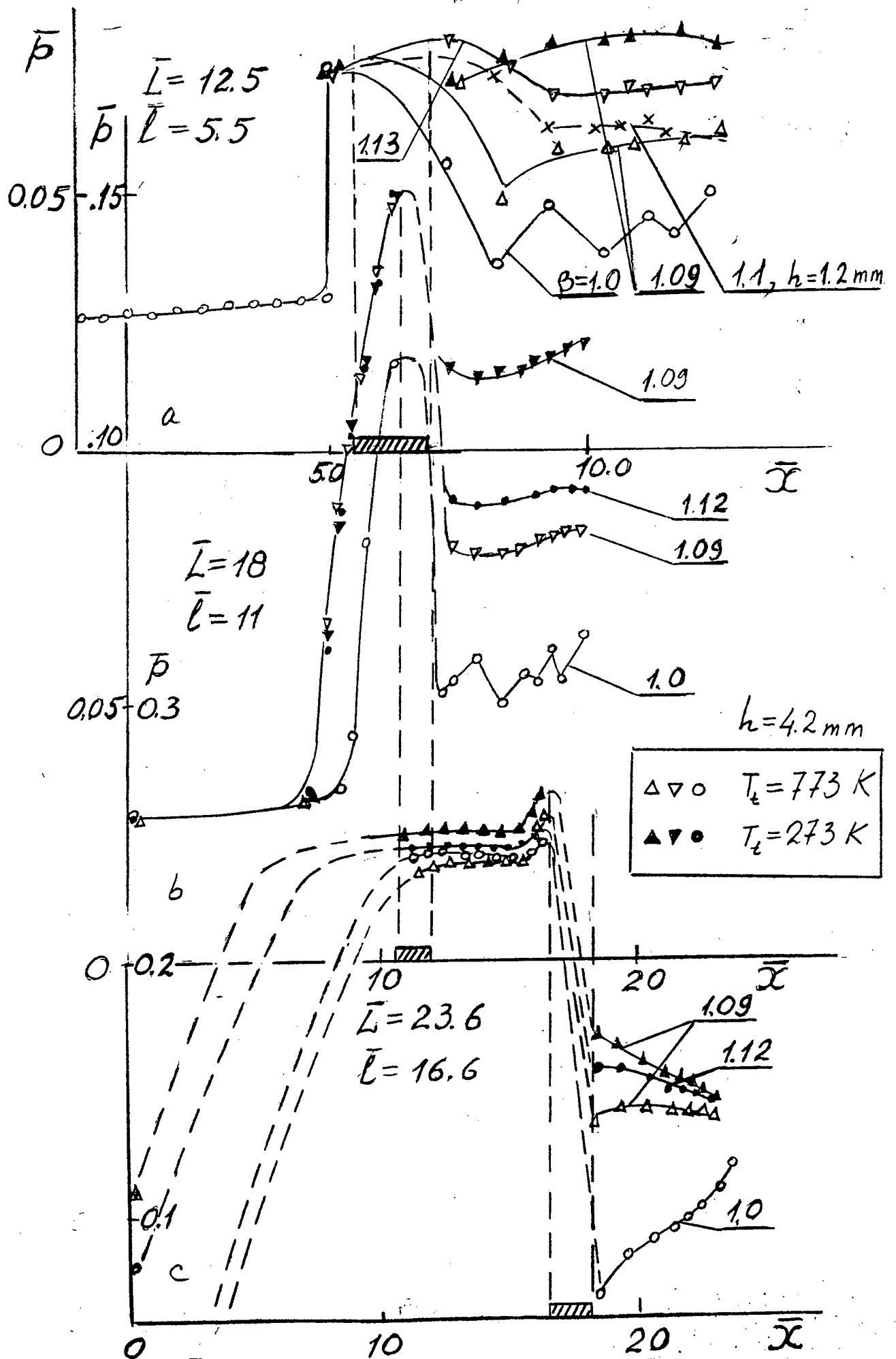
Fig.3.4.1 Pressure distribution in front of jet positioned at different parts of the tube and different \beta_{Tt} of jet
