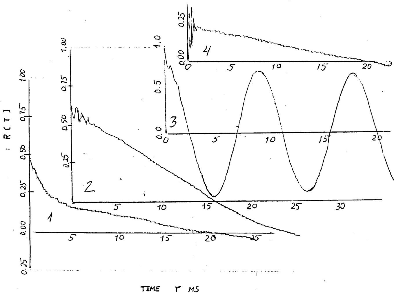
Fig. 3.5.20 Power spectra density vs. frequency. Autocorrelation function vs. time. cylindrical struts, 3 mm, 1- 1 row, 2 two rows, 3- three rows 4- one row, II section Ma=3.2, pseudo-shock, r.3, static pressure pulsations, I section
