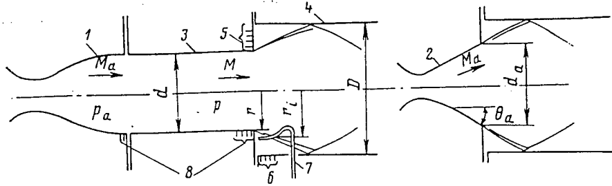
Fig. 4.2.1 Experimental module schematic.
