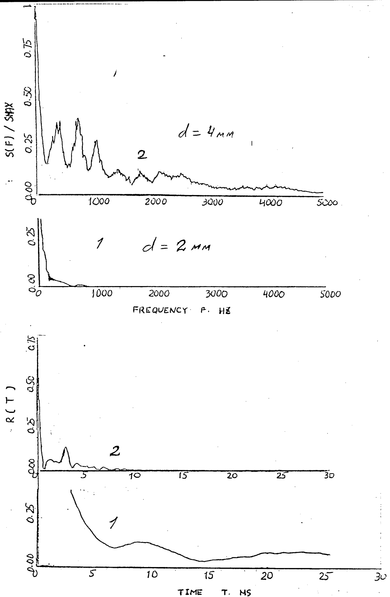
Fig.3.5.23 Power spectra density vrs. frequency. Autocorrelation function vrs. time. rhomb struts, - 1 row, Ma=3.2, pseudo-shock, r.3, total pressure pulsations, I section
