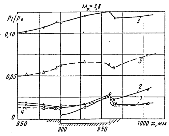
Fig. 3.3.6 Pressure distribution along the tube with a cavity.
