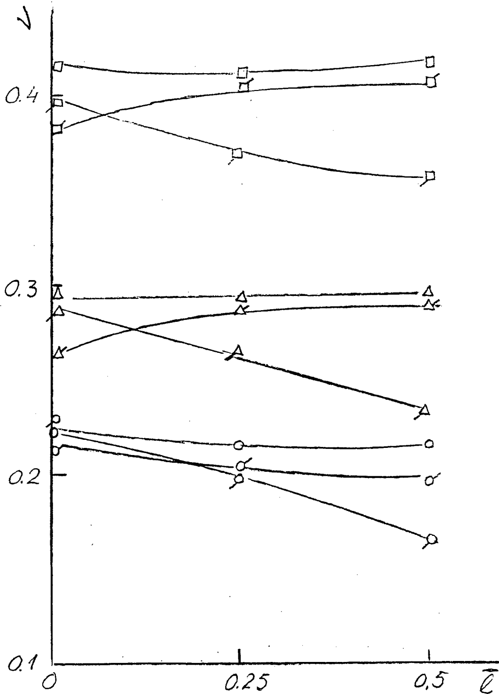
Fig. 3.1.9 Total pressure recoveries dependence on the gate width. Rhombic struts.
