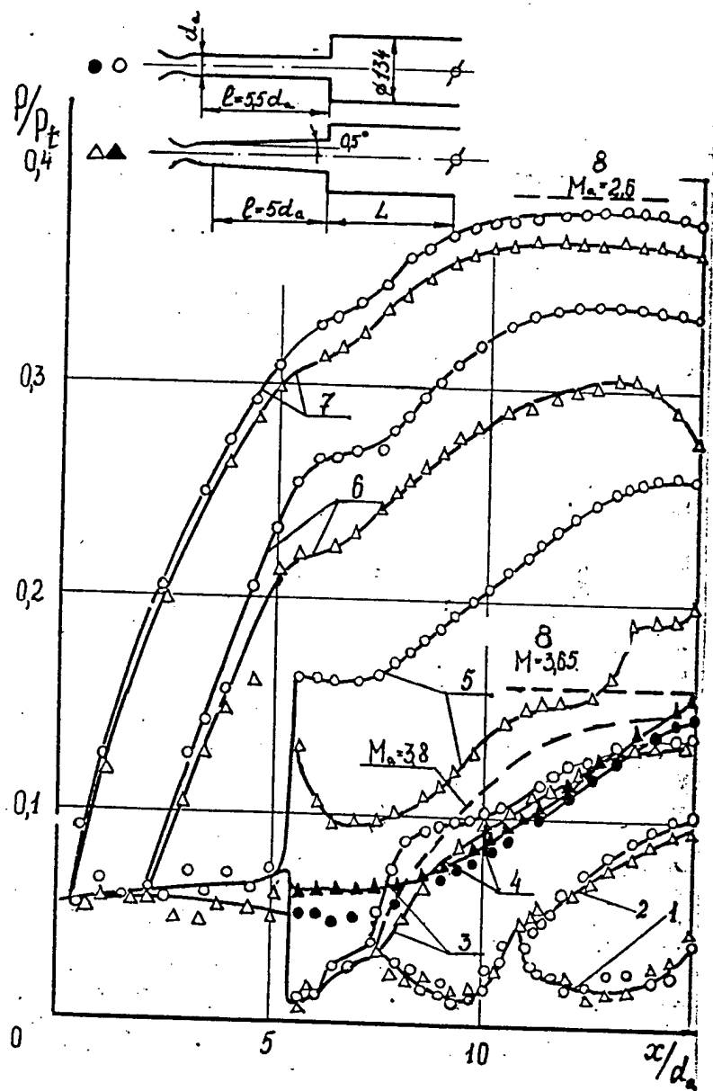
Fig. 4.5.1 Pressure distribution in stepped ducts at different back pressures. Ma=2.6 , 1-7-numbers of regimes, 8-normal shock, M=2.65 , 9- M=3.65
