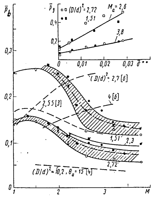
Fig. 4.2.8 Base pressure dependence on M
