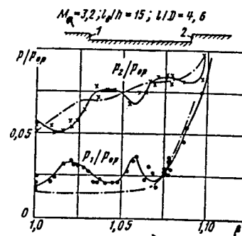
Fig. 3.2.5 Flow mode transformation due to jet injection in front of cavity.
