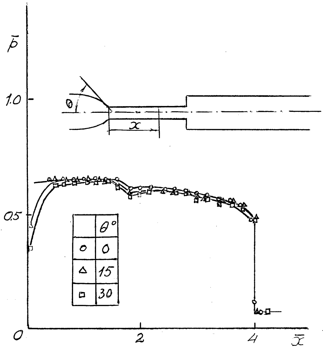
Fig. 4.2.10 Pressure distribution in tube downstream the sonic nozzle
