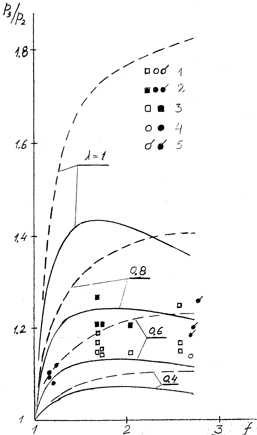
Fig. 4.7.5 Pressure recovery p_3/p_2 vs f in subsonic part of diffuser at different velocity coefficients \lambda in front of diverging section of the duct.
