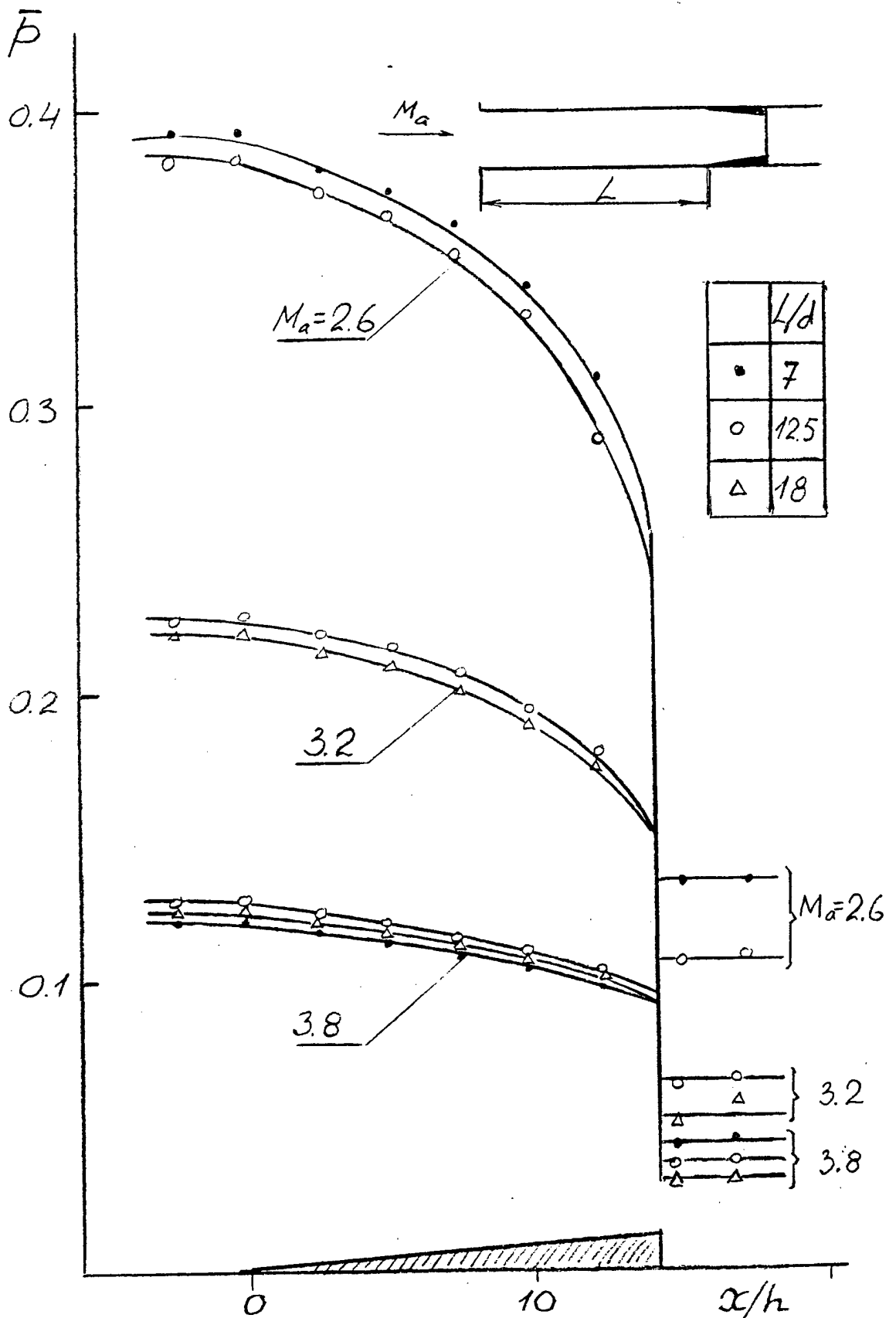
Fig. 4.2.1f Pressure distribution along the circular jut at different Ma and lengths of ducts installed between step and nozzle
