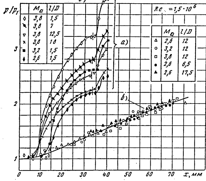
Fig. 2.1.1.1 Comparison of pressure distributions in front of the step and in pseudo-shock.
