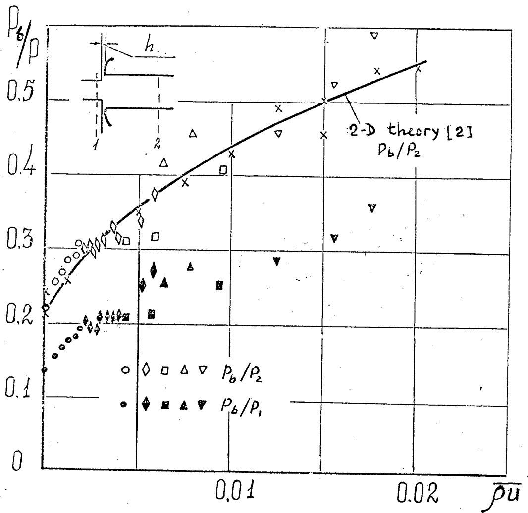
Fig. 4.2.18 Base pressure dependence on relative mass of jet injection into base region. Ma=2.6 , f=1.51
