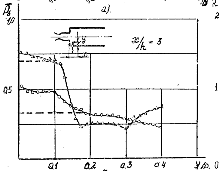
Fig. 4.5.2 Pressure profiles measured by Pitot tube downstream the step. ○ △ correspond to curves 3, ● ▲ -4 of Fig 4.5.1
