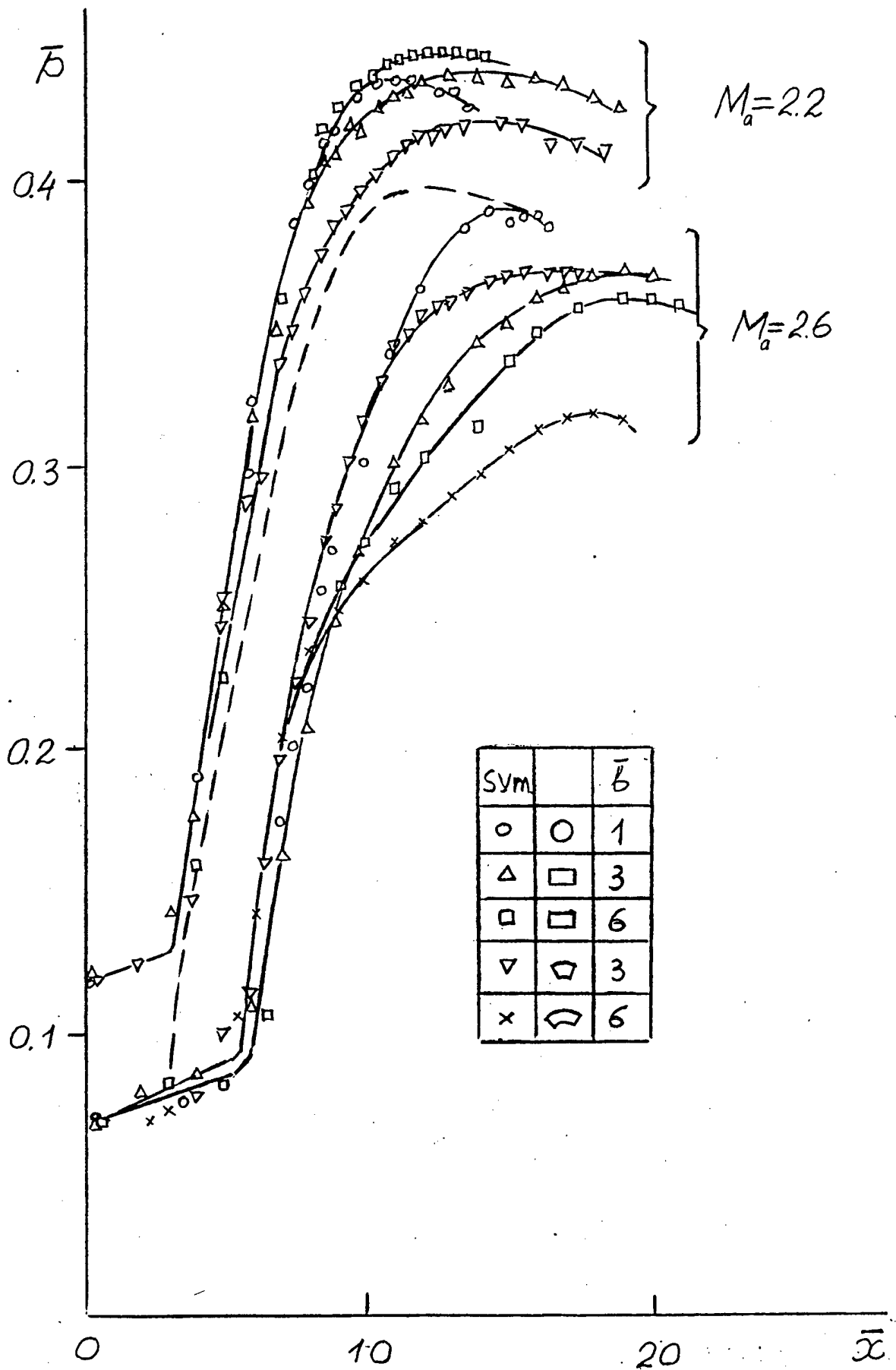
Fig.2.3.2 Pressure distribution at maximal back pressure. Second, basic stage of flow. Ma=2.2, 2.6
