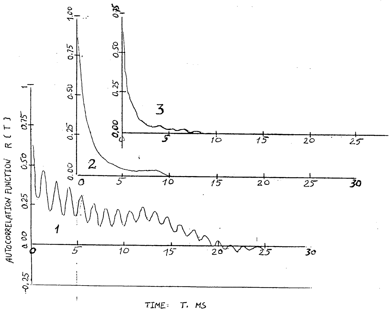
Fig.3.5.10 Power spectra density vrs. frequency. Autocorrelation function vrs. time. 1- no struts, 2- rhomb struts, 1 row, 3- cilindric struts, 1 row Ma=3.8 , supersonic flow, static pressure pulsations, I section
