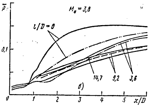
Fig. 3.3.4 Pressure distribution along tubes with obstacles. 1-obstacle removed.
