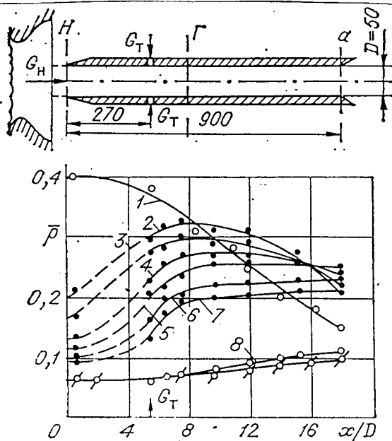
Fig.2.1.1.12 Pressure distribution in cylindrical duct in free stream, Ma=2.5 at different supplies of gas from generator 1- \beta=1.03 , 2-1.22, 3-1.019, 4-1.016, 5- 1.015 6-1.012, 7-1.009, 8-1.0
