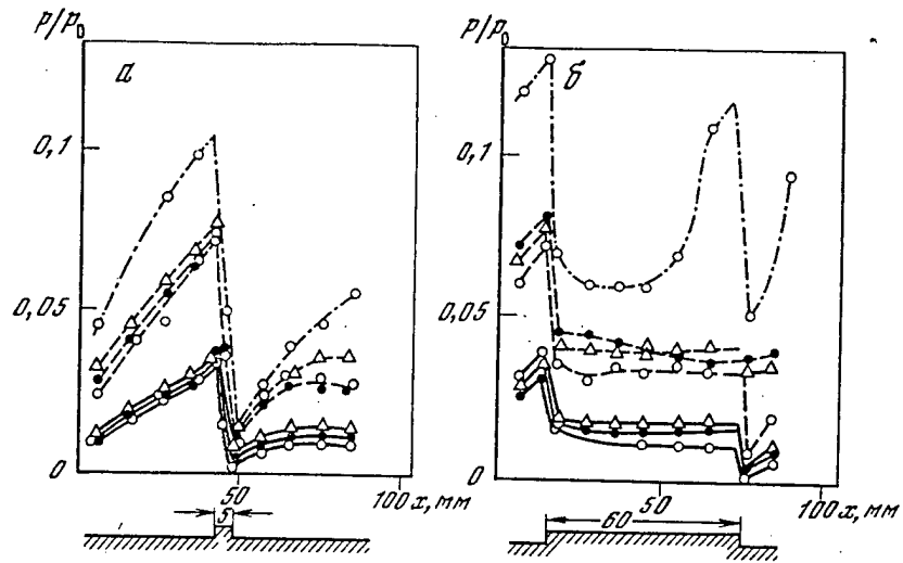
Fig. 3.1.4 Pressure distribution along the annular jet. a- jut length-5 mm, b-60 mm. Open circles for x/D = 0.7 shaded-4.4 mm, open triangles-10. Solid line for Ma = 3.8 , dashed-3.2, dashed-dotted-2.6.
