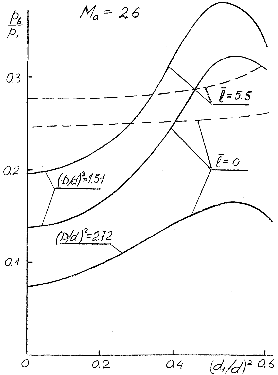
Fig. 4.4.4 Annular duct base pressure dependence on (\frac{d_1}{d})^2 M_a=2.6 ,—annular stepped duct, ---plane step
