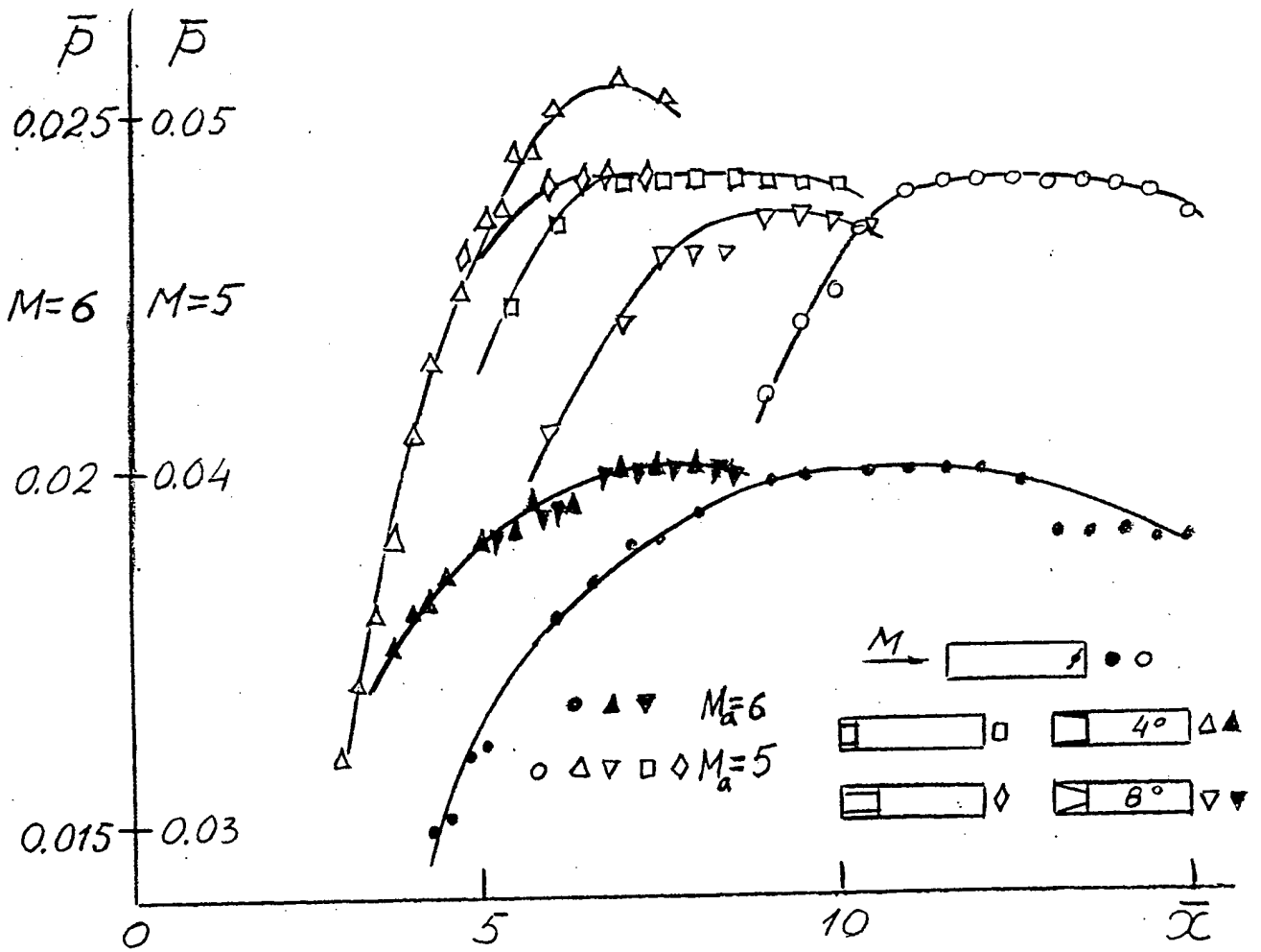
Fig. 3.3.7 Pressure distribution along rectangular duct with wedges installed on the walls.
