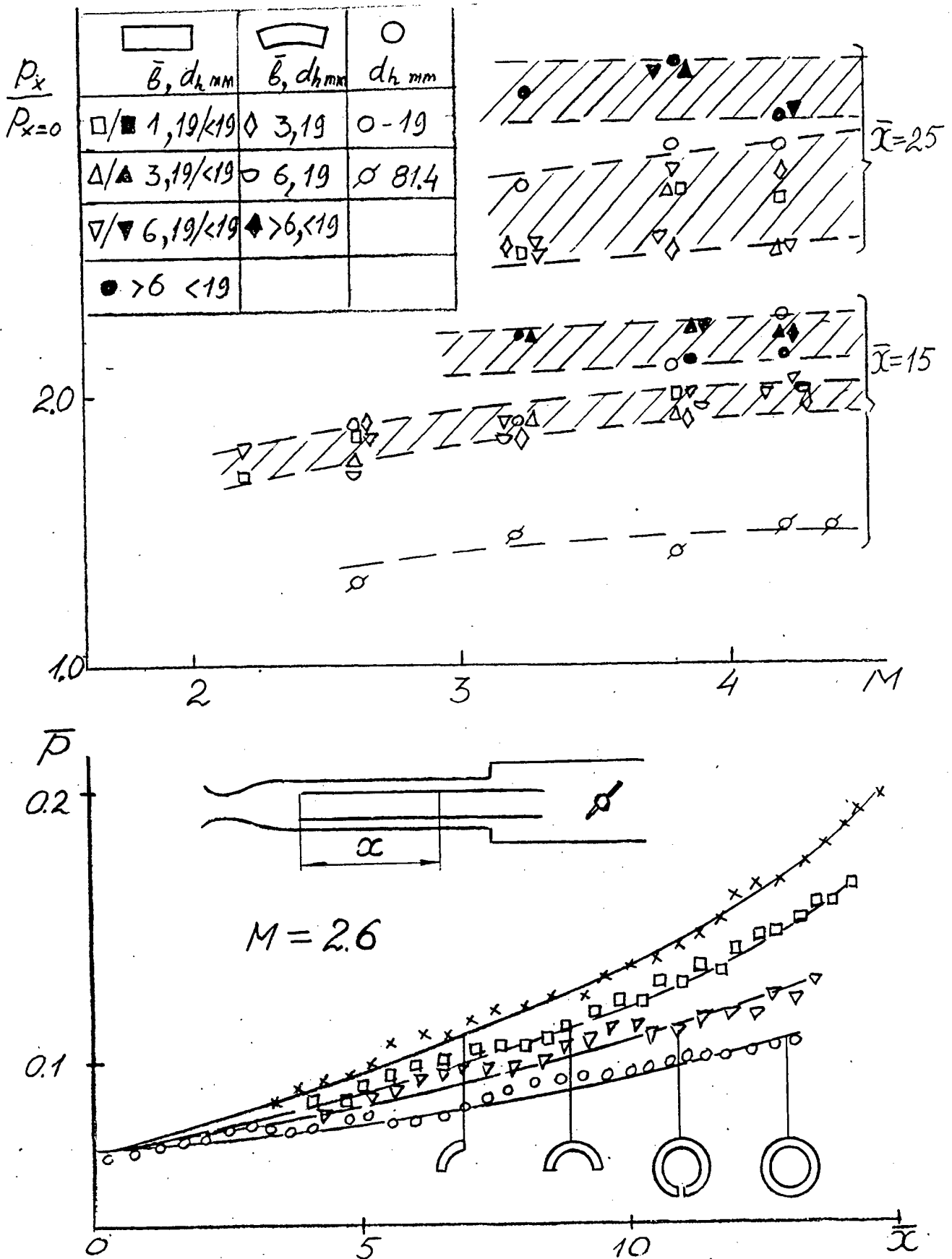
Fig. 2.3.1. a) P_x/P_{x=0} dependence on Ma . initial stage, supersonic duct flow, Ma=3.8 , b) Pressure distribution along annular sector duct, Ma=2.6 .
