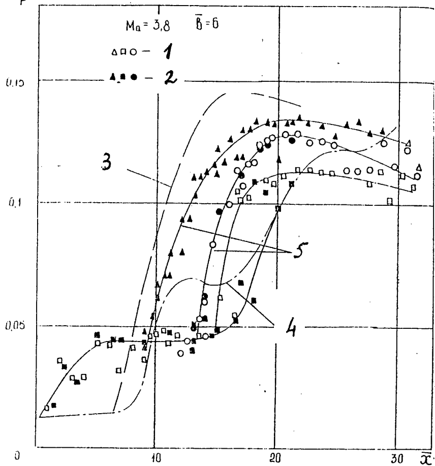
Fig. 5.2.1 Transformation of separation flow into pseudo-shock due to variation of cross section shape along the duct length, b=6 , M_a=3.8 1-wide, 2-narrow walls, 3-circular, 4-rectangular duct
