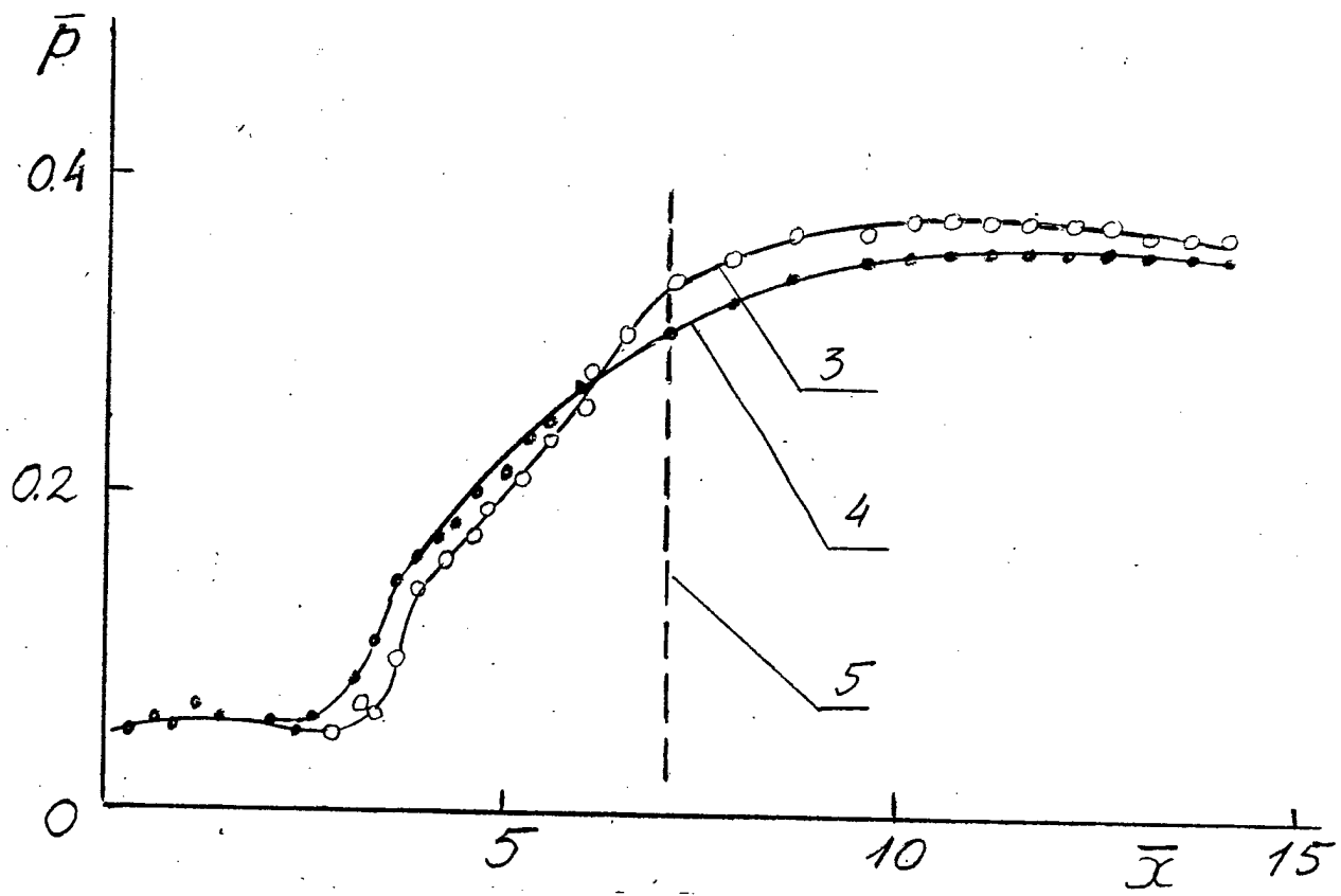
Fig.2.2.1.16 Comparison of pressure distribution along pseudo-shock with and no bleeding. 1-bleeding section, 2-rate meter, 3-no bleed, 4-bled, 5-section of bleeding.
