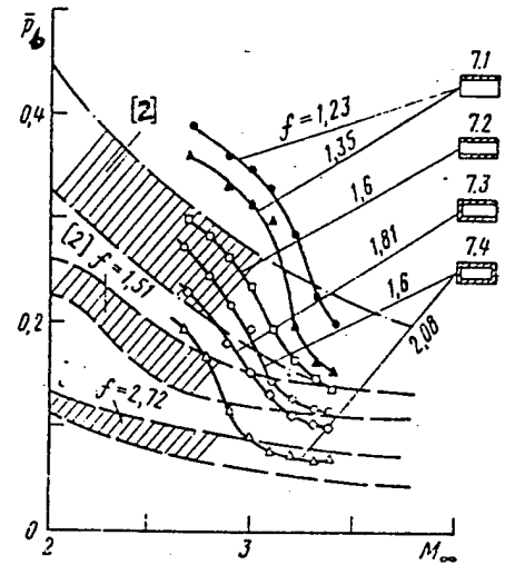
Fig. 4.3.4 Base pressure dependence on M_\infty
