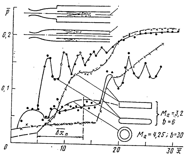
Fig. 2.1.2.2 Pressure distribution in ducts with oblong cross sections. 1—plane or sector duct, 2—annular duct.
