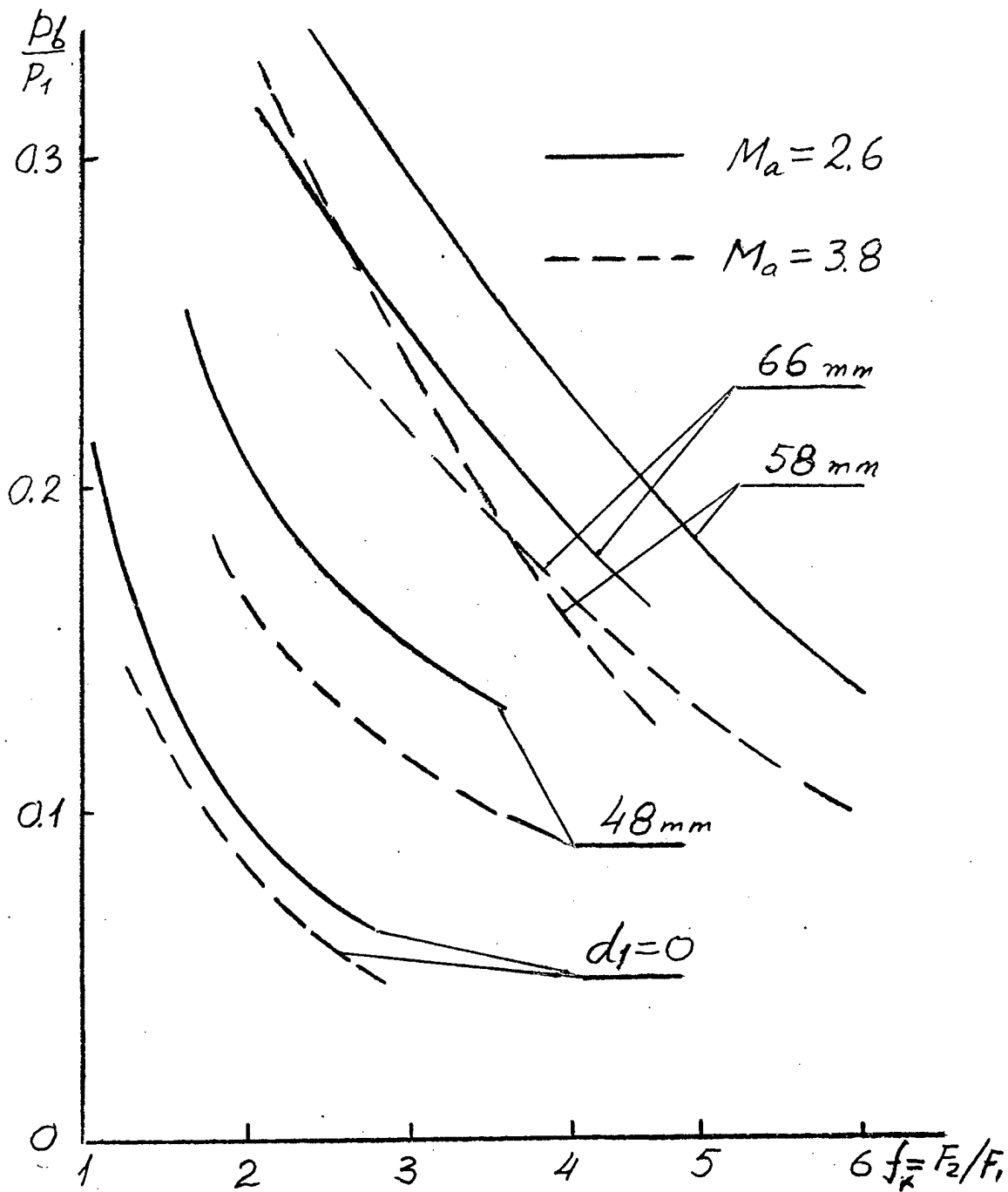
Fig. 4.4.6 Annular duct base pressure dependence on f_2 Ma=2.6 , — annular stepped duct, - - - annular duct
