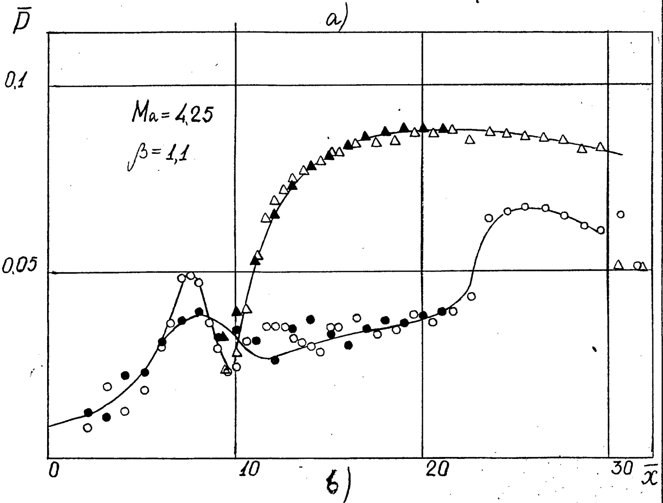
Fig. 2.2.2.11 Pressure distribution at jet injection from the wall, Ma=4.25 , b=6 .
