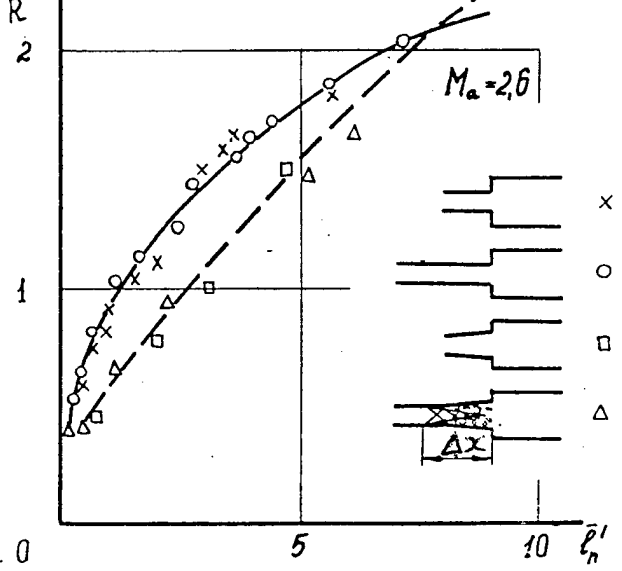
Fig. 4.5.4 Distances of upstream influence vs. back pressure M_a = 2.6 , — \bar{l} = 11 , --- \bar{l} = 0 , 1-6- numbers of regimes, 7-wide part, 8- narrow part of the stepped duct.
