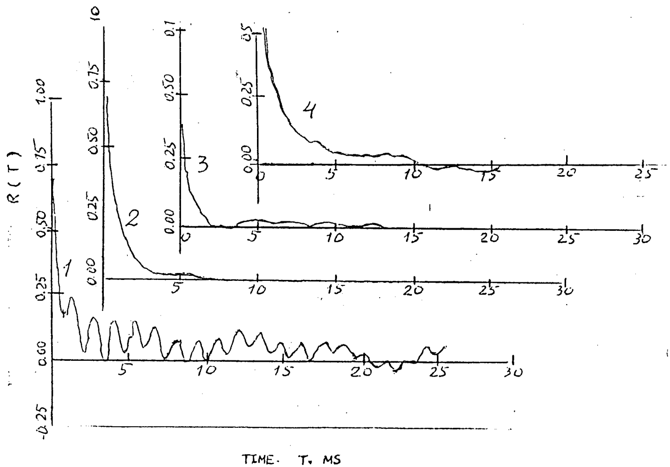
Fig 3.5.14 Power spectra density vs. frequency. Autocorrelation function vs. time. rhomb struts, 3 mm, 1- 1 row, 2 two rows, 3- three rows 4- one row, II section Ma=3.2 , supersonic flow, static pressure pulsations, I section
