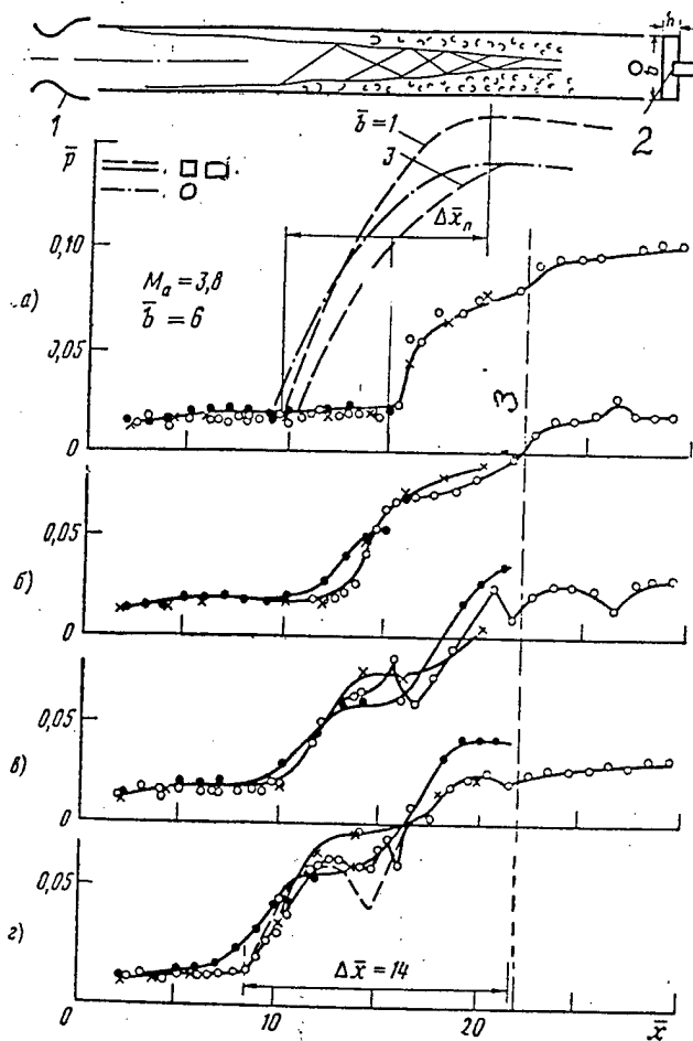
Fig. 2.1.2.1 Pressure distribution in pseudo-shock in rectangular duct, b = 6 , Ma = 3.8 . ----, —, rectangular duct. —●— circular duct, ○—wide wall, ●—narrow wall (right), x—(left), 1—nozzle, 2—throttle, 3—rake P_t^1
