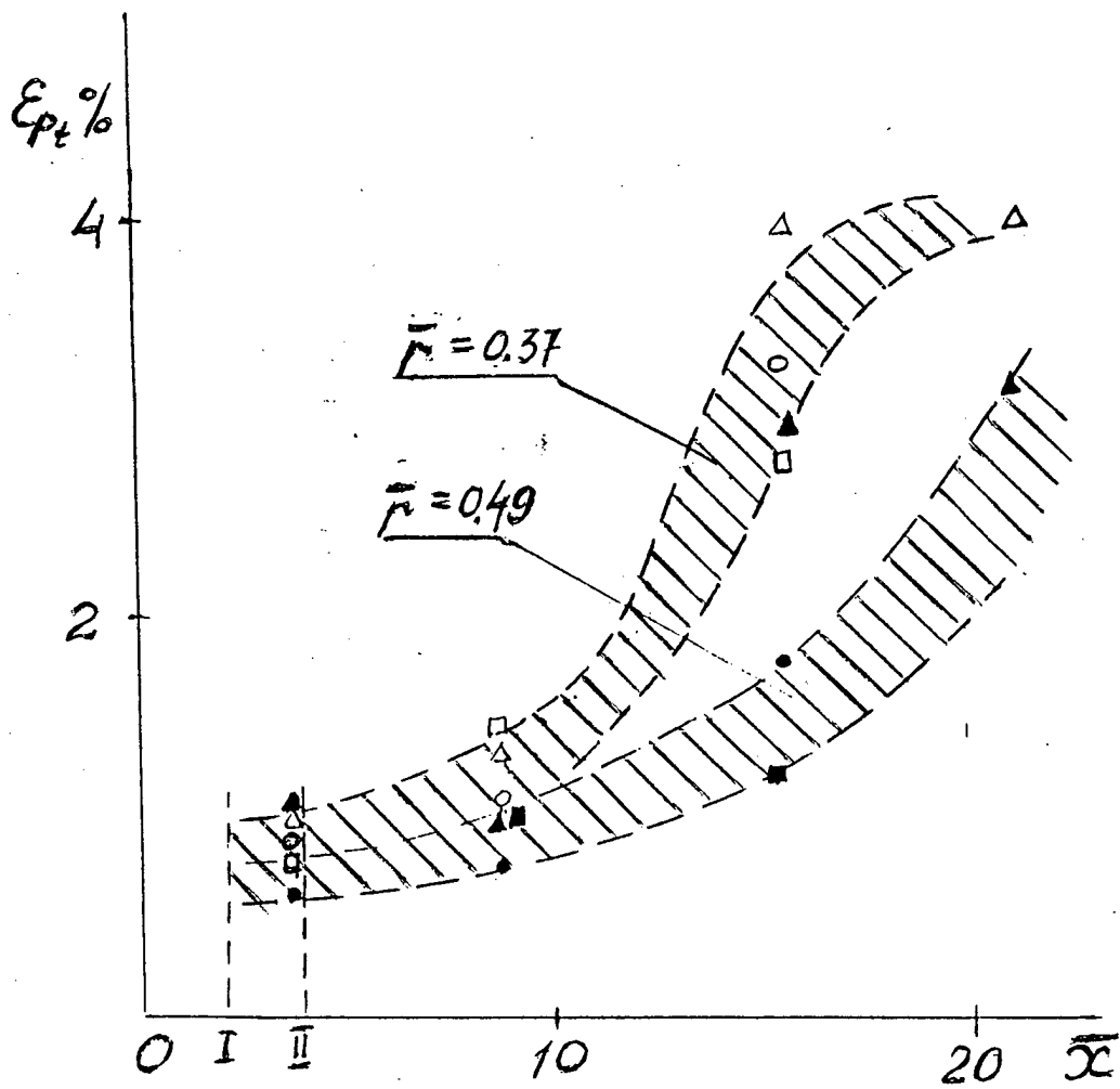
Fig.3.5.6 Total pressure pulsation intensity - \epsilon_{p_t} along the tube at two distances from the wall. smooth tube, \circ \text{Ma}=2.6 , \square \text{Ma}=3.2 , \triangle \text{Ma}=3.8
