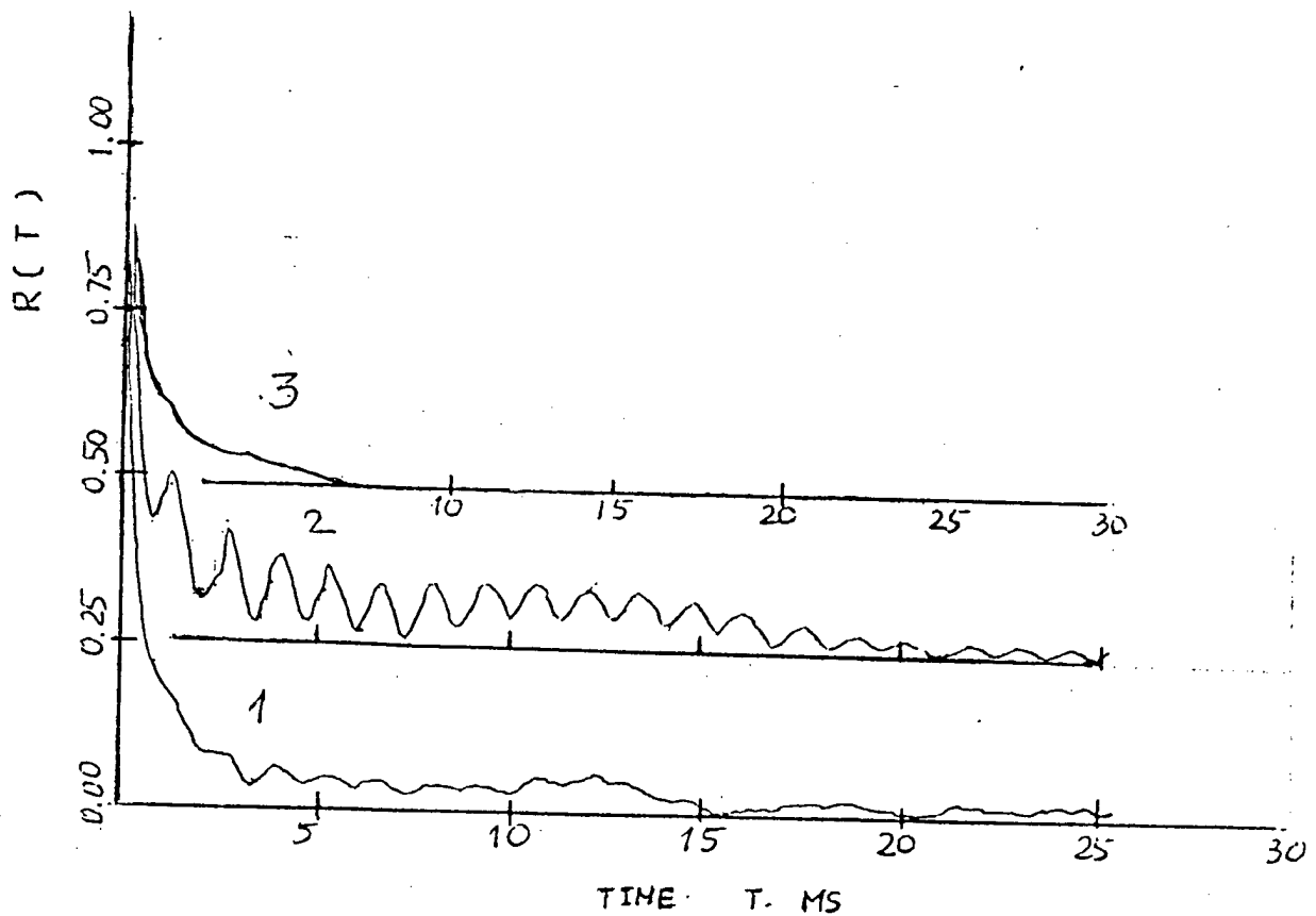
Fig.3.5.18 Power spectra density vs. frequency. Autocorrelation function vs. time. cylindrical struts, 3 mm, 1- 1 row, 2 two rows, 3- three rows 4- one row, II section Ma=3.2, supersonic flow, static pressure pulsations, I section
