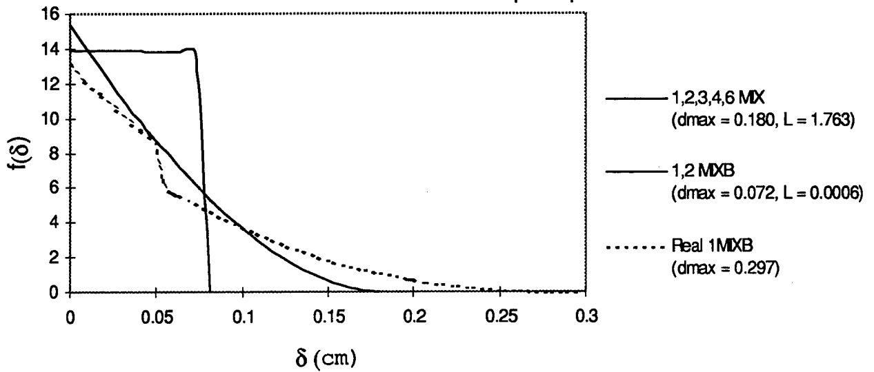
Figure D-10: Two parameter, multiexperiment results for MIX sizes
