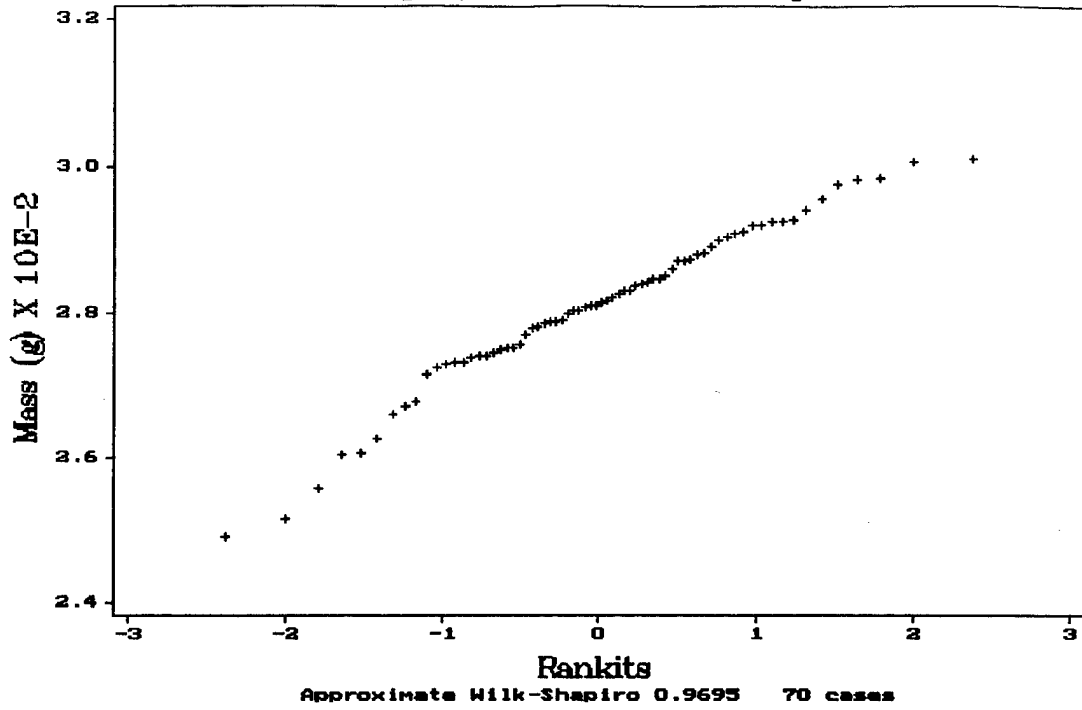
Figure 6.: Normal probability plot for small paraffin spheres
