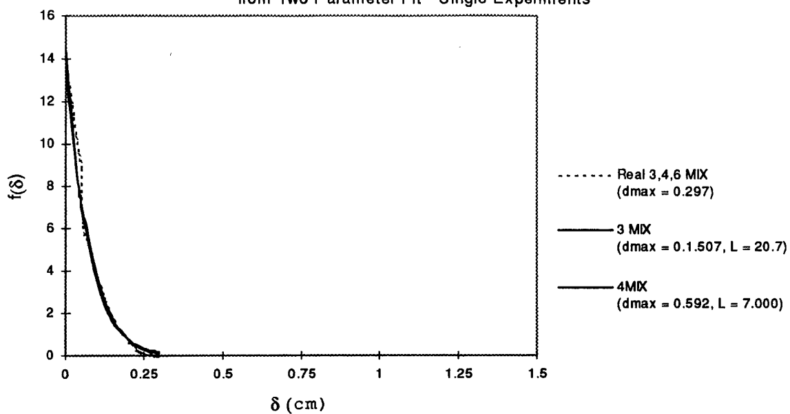
Figure: D-13: Two parameter single experiment results for 3 and 4 MIX, full scale
