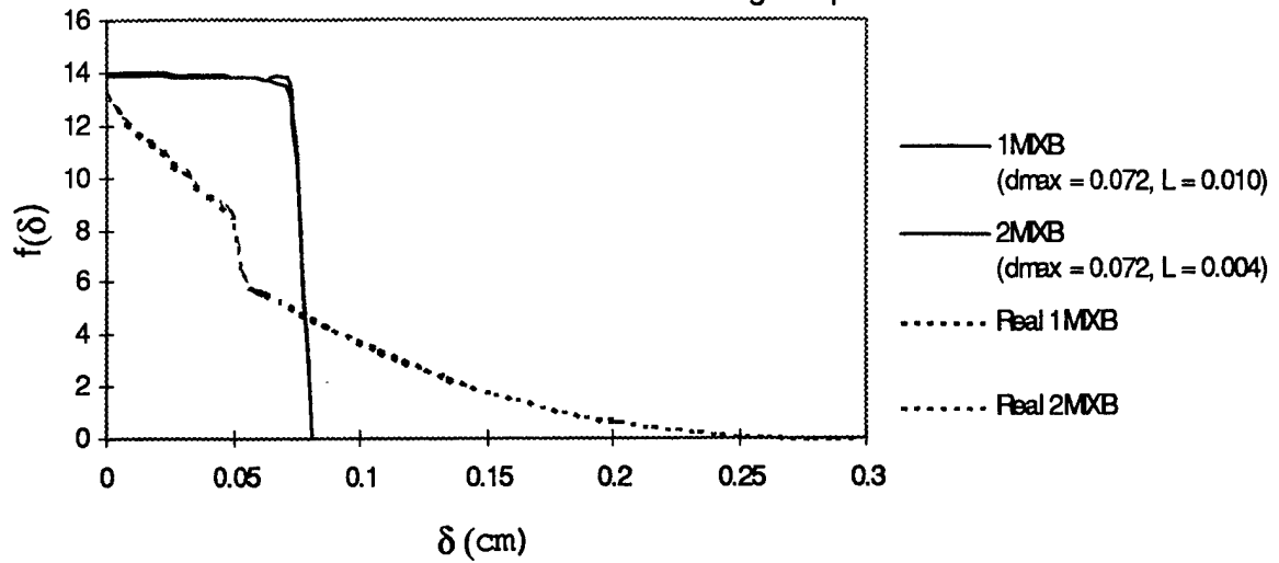
Figure D-9: Two parameter, single experiment results for 1-2 MIX
