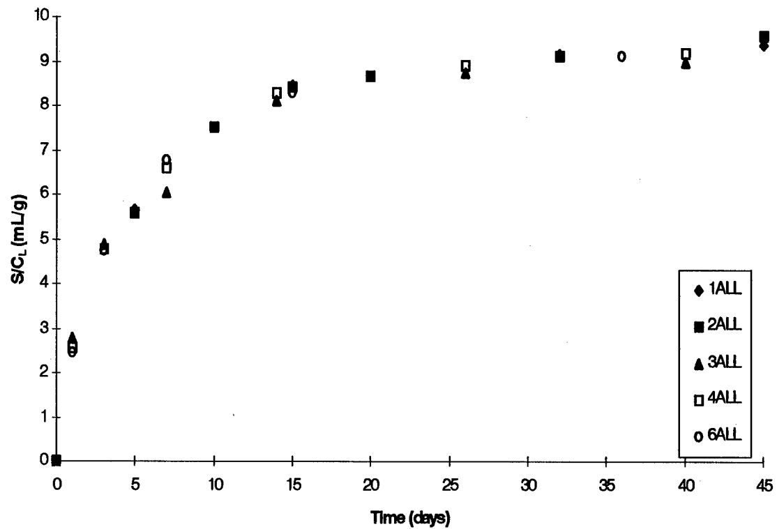
Figure C-5: ALL paraffin spheres sorption rate
