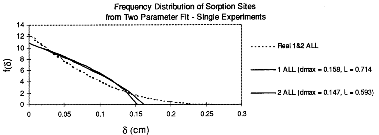
Figure D-5: Two parameter fit results for MSS using single experiment data, 1-2 ALL
