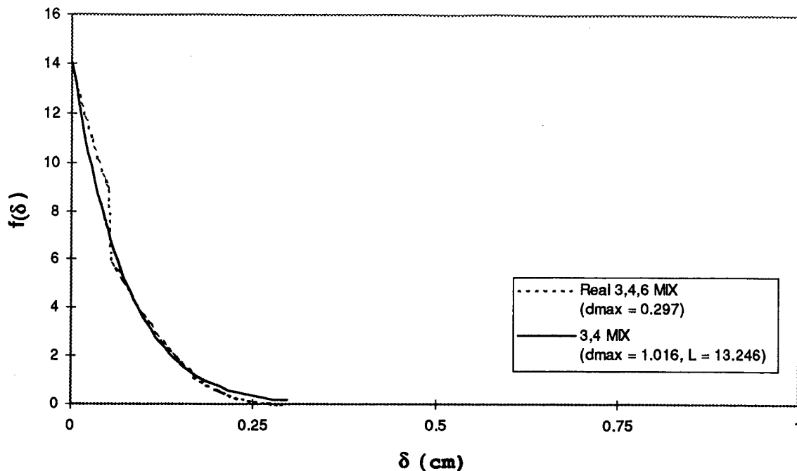
Figure 14: Frequency distribution of sorption sites using fitted \delta_{max} ( d_{max} ) and \lambda (L)
