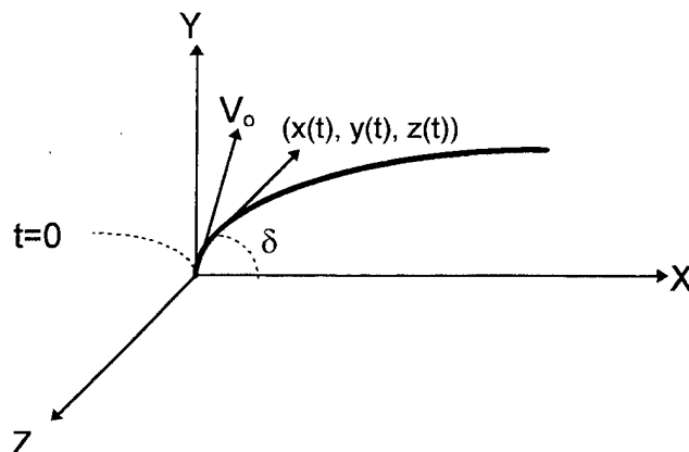
Figure 11. Projectile location at time t
