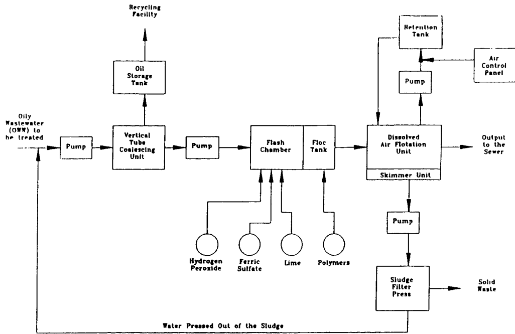
Figure 5. U.S. Navy Oil Wastewater Treatment Plant (Nuckols et al. 1994).
