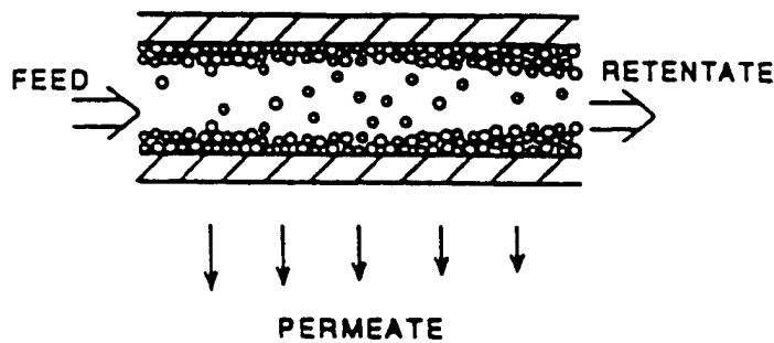
Figure 7. Crossflow Microfiltration (Davis 1992).
