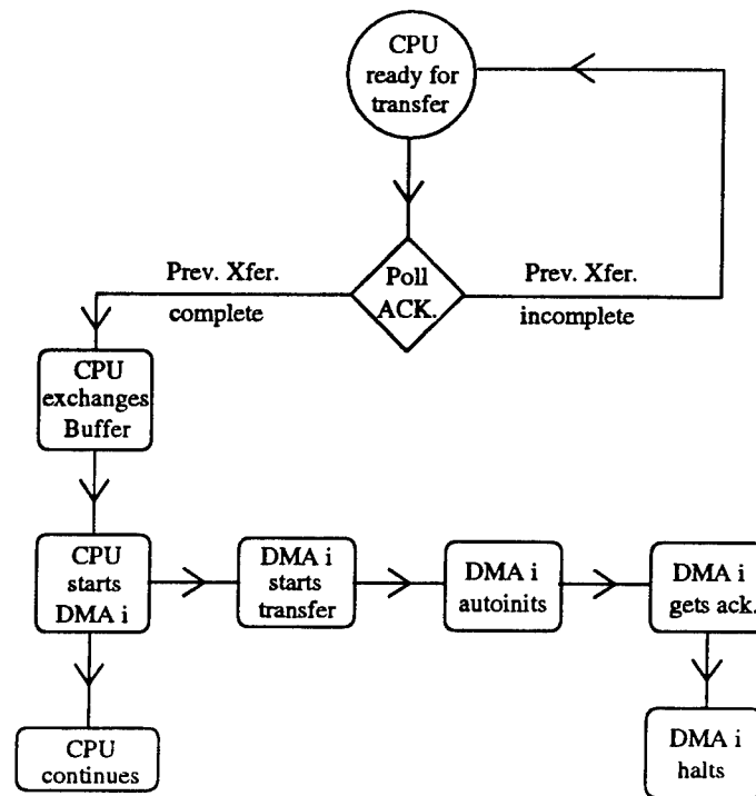
Figure 8: CPU-DMA Interactions for SIPC
