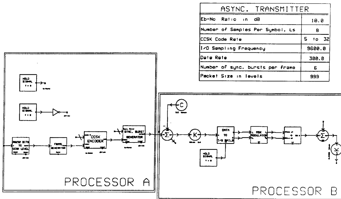
Figure 4: SPW System: "mpxmit2.system"
