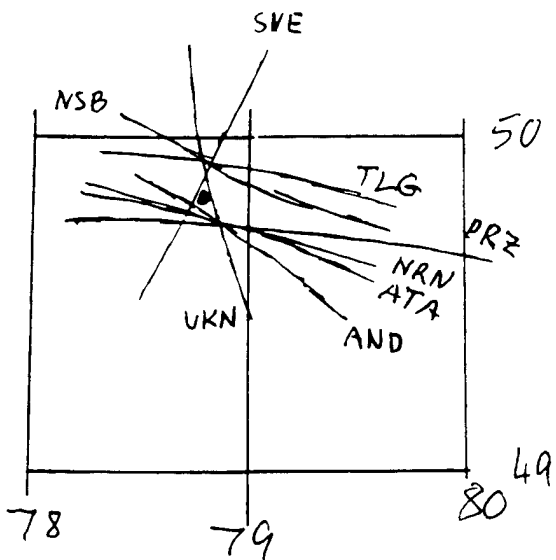
1987-Sep-16 (49.85°, 78.79°) (6.7 km, 12.7 km)
