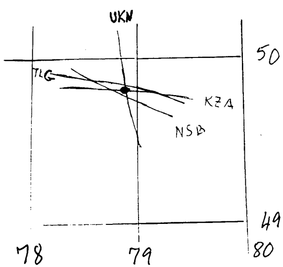
1981-Jun-05 (49.80°, 78.86°) (7.9 km, 15.5 km)
