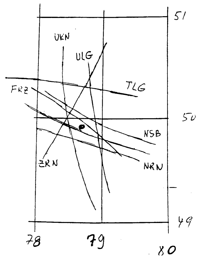
1988-Sep-26 (50.10°, 78.96°) (18 km, 16 km)
