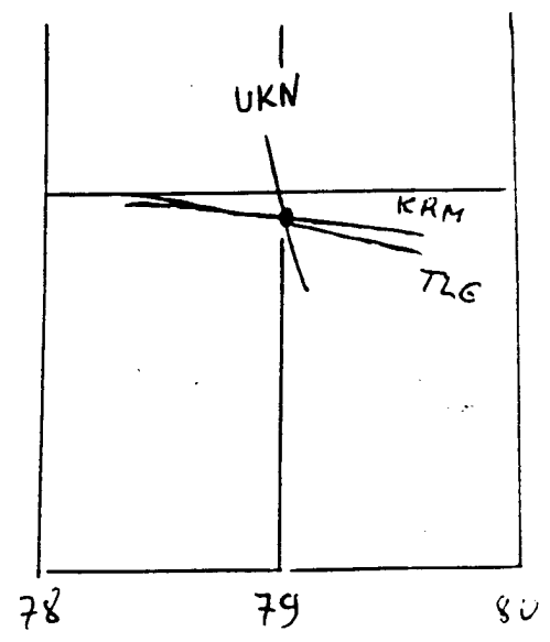
1984-Jun-23 (49.93°, 79.01°) (2.2 km, 4.5 km)
