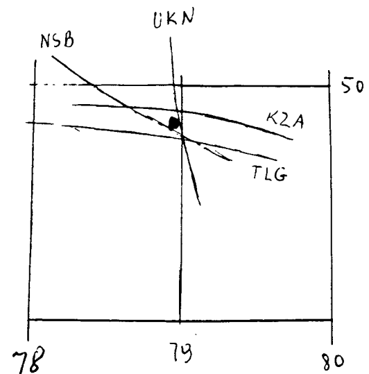
1981-Jul-05 (49.85°, 78.90°) (6.3 km, 10.5 km)
