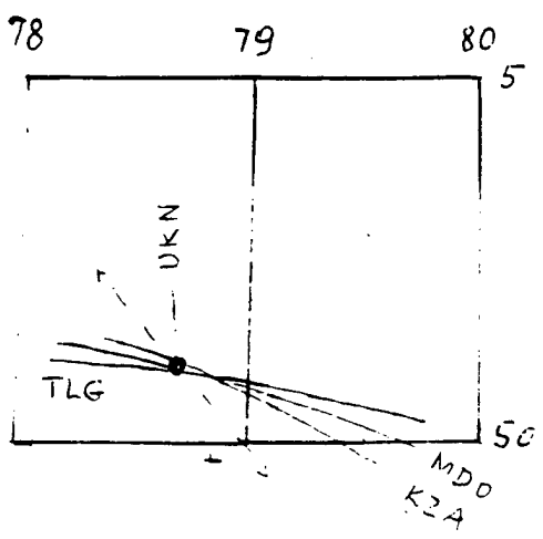
1981-Nov-19 (50.20°, 78.71°) (10 km, 10 km)
