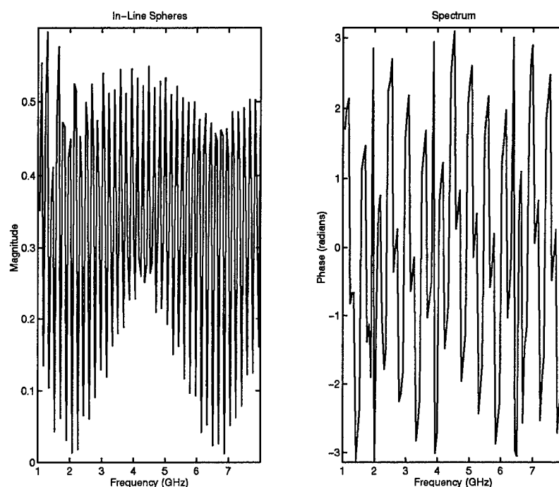
Figure 3.9: In-Line Spheres: Spectral Response
