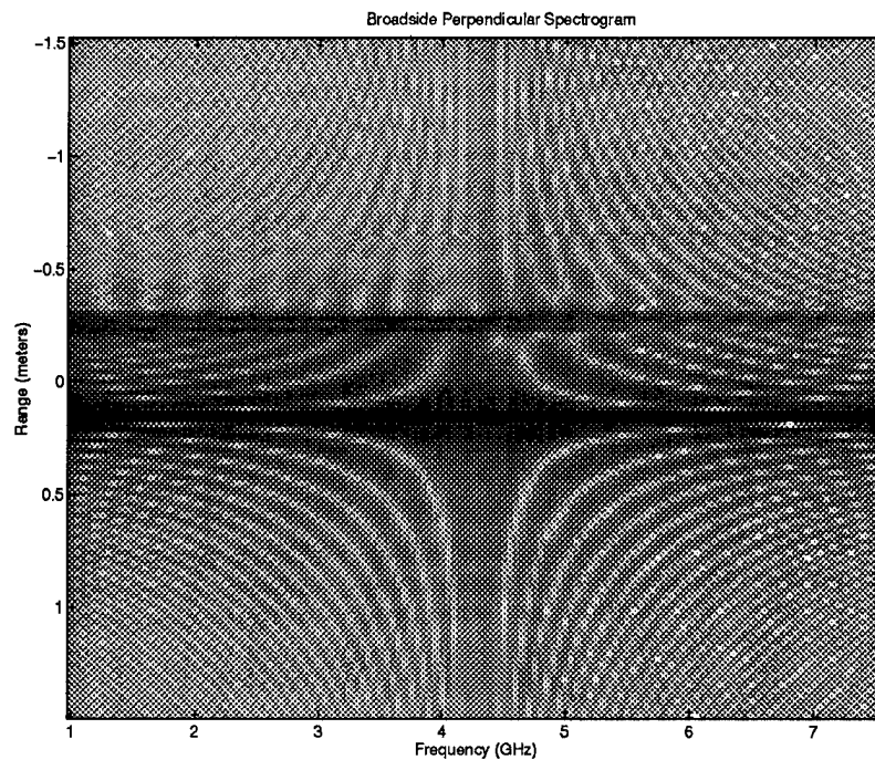
Figure 3.16: Broadside — Perpendicular Polarization: Spectrogram
