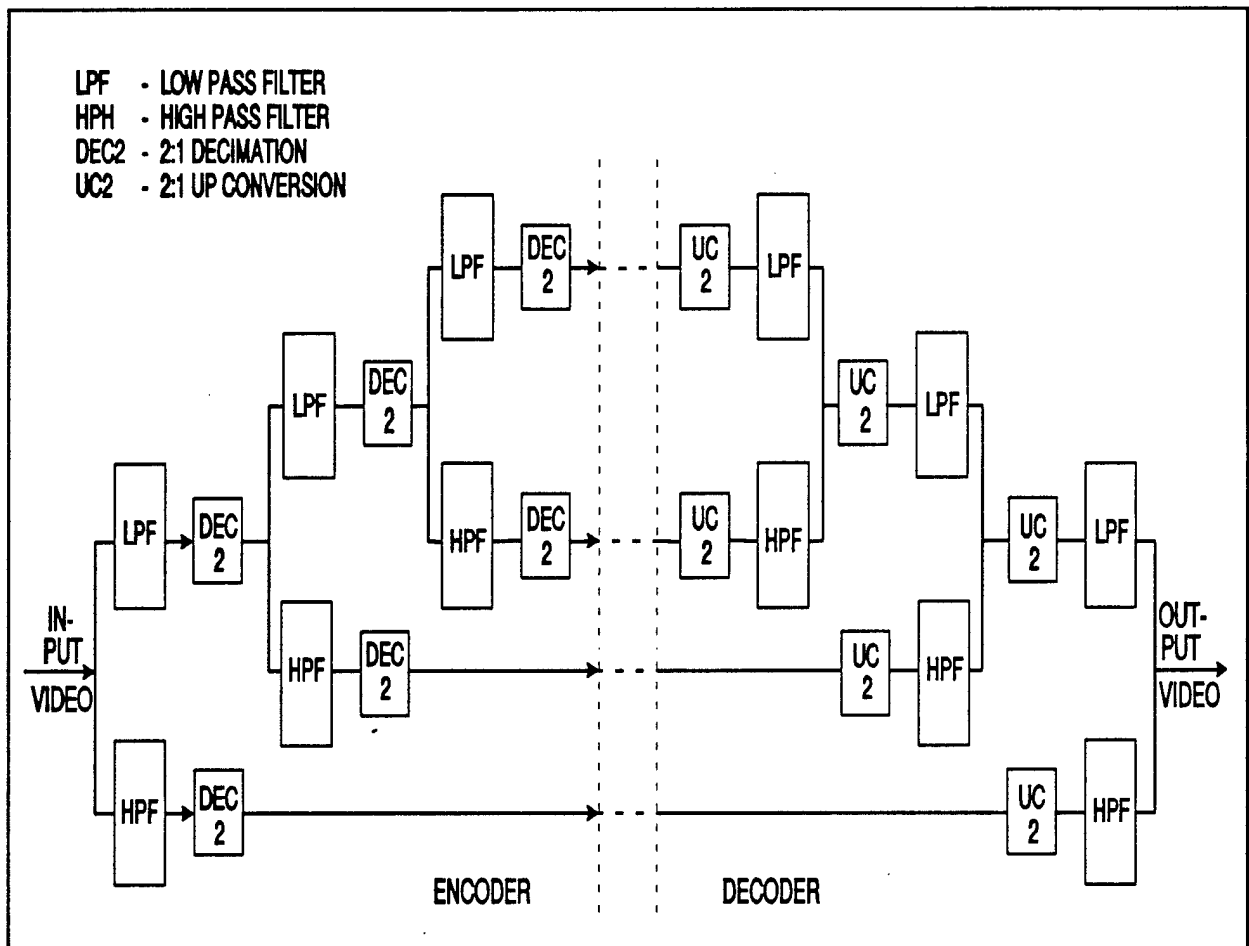
FIGURE 4.1 FUNCTIONAL BLOCK DIAGRAM OF A TYPICAL WAVELET CODEC
