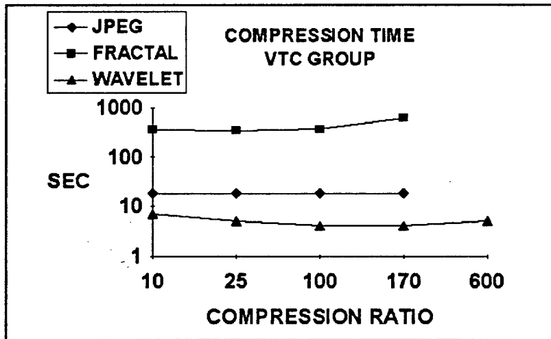
FIGURE 7.4 COMPLEXITY RESULTS - VTC GROUP
