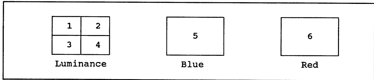
FIGURE 2A.3 ARRANGEMENT OF BLOCKS IN A MACROBLOCK
