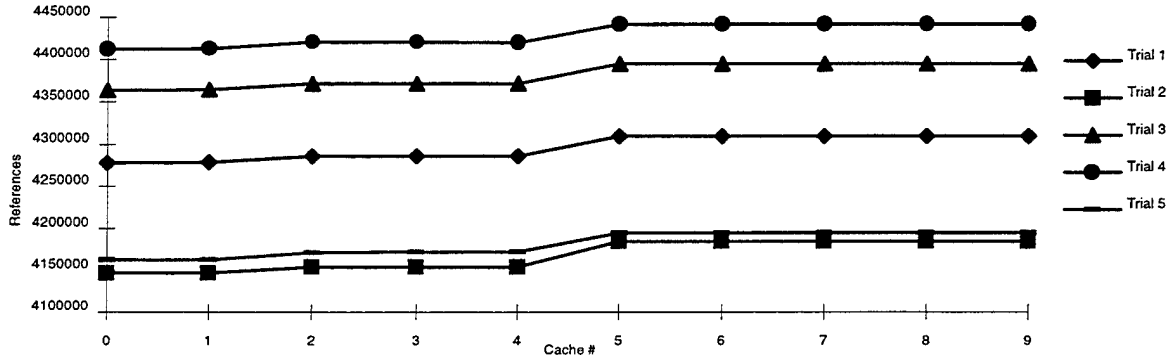
Figure 3: Operating System Instruction Fetches Within Same Program Execution
