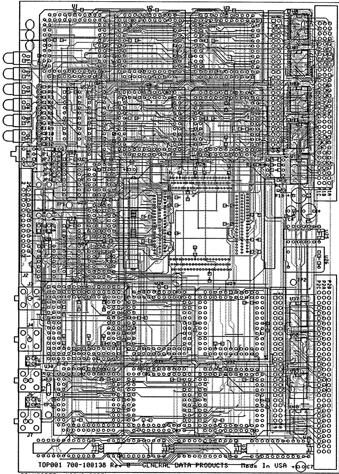
SILKSCREEN (COMP SIDE)
