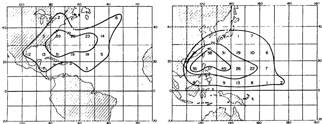
d) Distribution of western Pacific looping storms per 10° Marsden square per 21 years.
