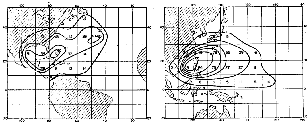
b) Distribution of western Pacific slow moving storms per 10° Marsden square per 21 years.
