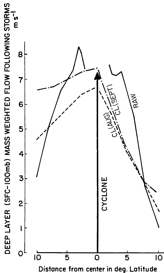
Figure 4.3: c. Same as Fig. 4.3a, but for the Atlantic All Northeast movers. All dashed lines reflect cross sections centered at 35^{\circ}N, 75^{\circ}W . On the left side facing the direction the TCs move, the cross section is directly west to 35^{\circ}N, 85^{\circ}W . To the right of the TC track facing the direction the TCs move, the cross section is toward the southeast to 30.5^{\circ}N, 61^{\circ}W .
