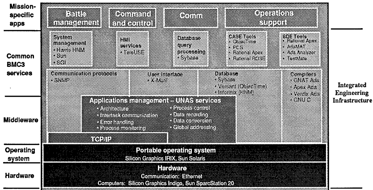
Figure 2. CI-1 Product Components
