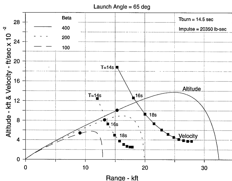
Figure 5. Representative PMI flyout trajectory with standard ASAS motor at 14.5 sec burnout and 65 degree launch angle.
