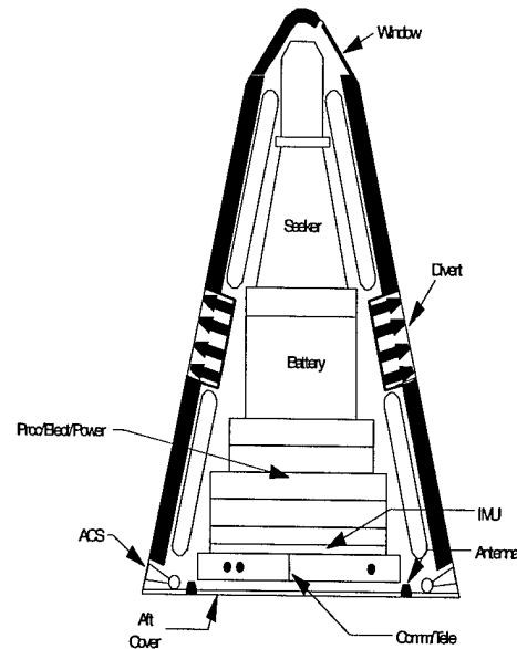
Figure 8. Schematic of active homing endgame design option front-end kill vehicle.
