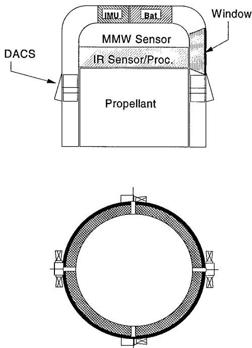
Figure 9. Schematic of hover endgame design option front-end kill vehicle.
