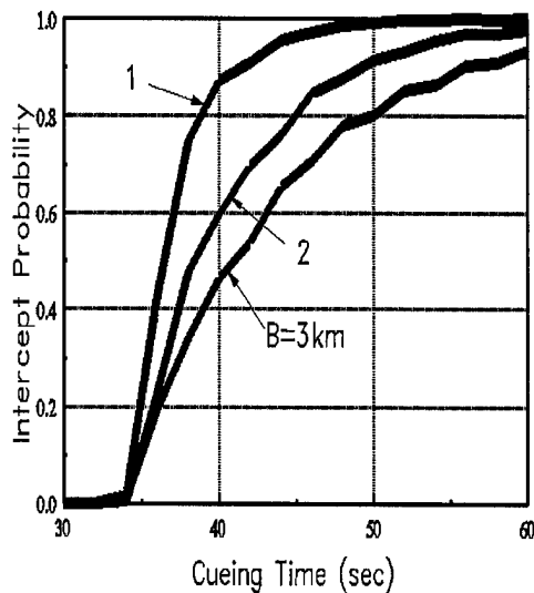
Figure 12. Probability of cruise missile intercept by a single PMI for the homing endgame option for several values of the cueing uncertainty in the predicted target position
