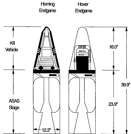
Figure 4. Schematic of PMI with ASAS motor propulsion and hover endgame and homing endgame front-end options.
