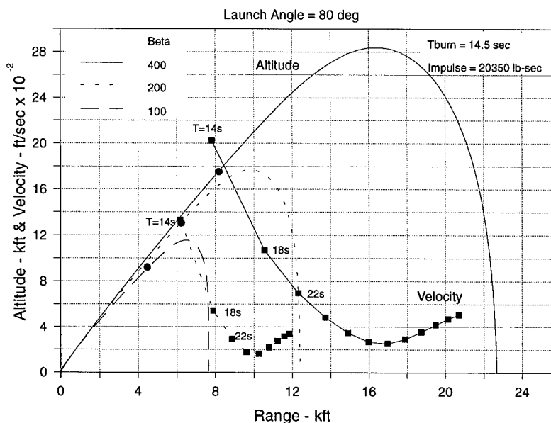
Figure 6. Representative PMI flyout trajectory with standard ASAS motor at 14.5 sec burnout and 80 degree launch angle.
