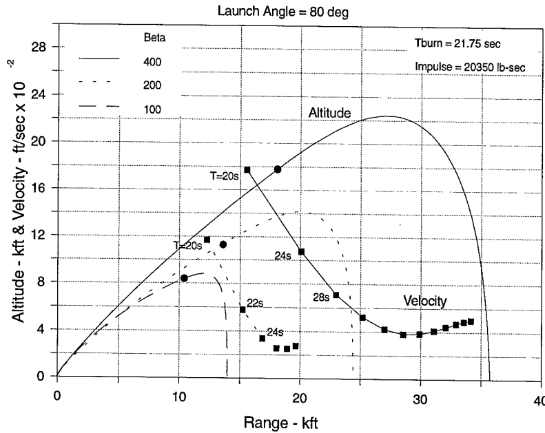
Figure 7. PMI flyout trajectory with ASAS motor at 21.75 sec burnout and 80 degree launch angle.
