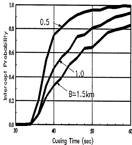
Figure 11. Probability of cruise missile intercept by a single PMI for the hover endgame option. The parameter B is the cueing uncertainty in the predicted target position
