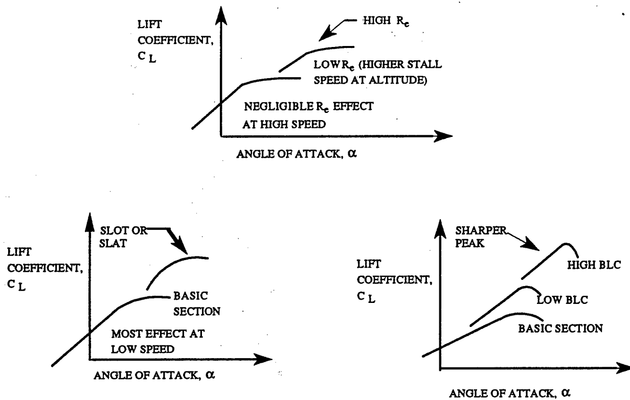
FIGURE 10.2. SEPARATION EFFECTORS
