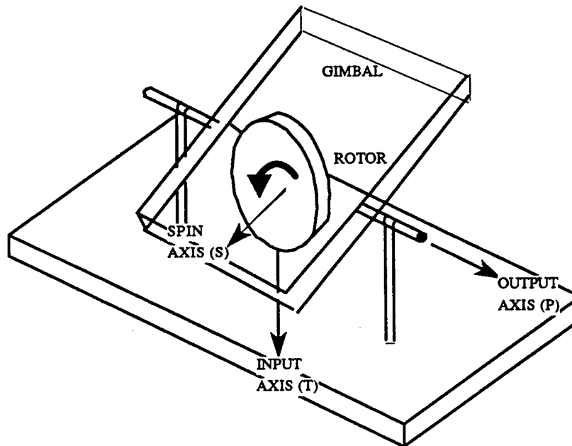
FIGURE 10.28. GYROSCOPE AXES
