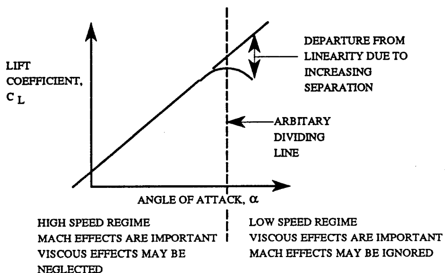
FIGURE 10.1. SEPARATION
