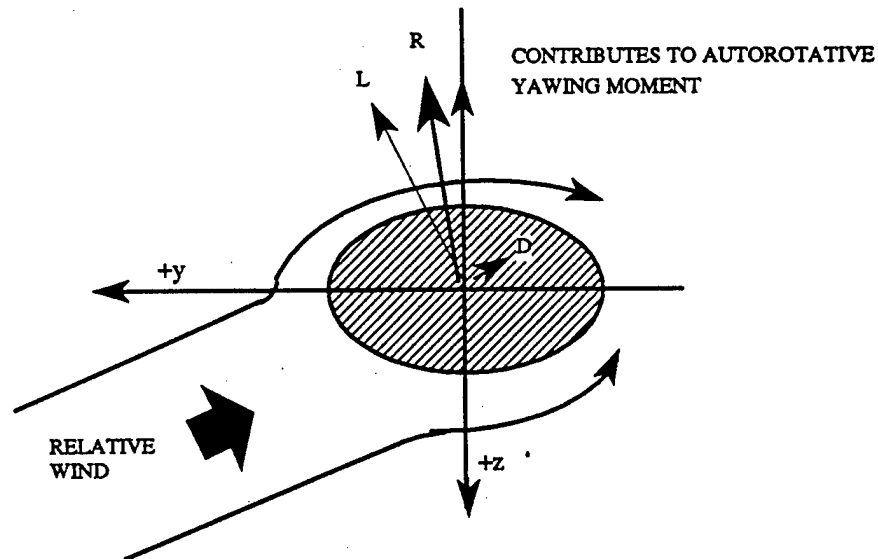
FIGURE 10.20A. PLAIN FUSELAGE
