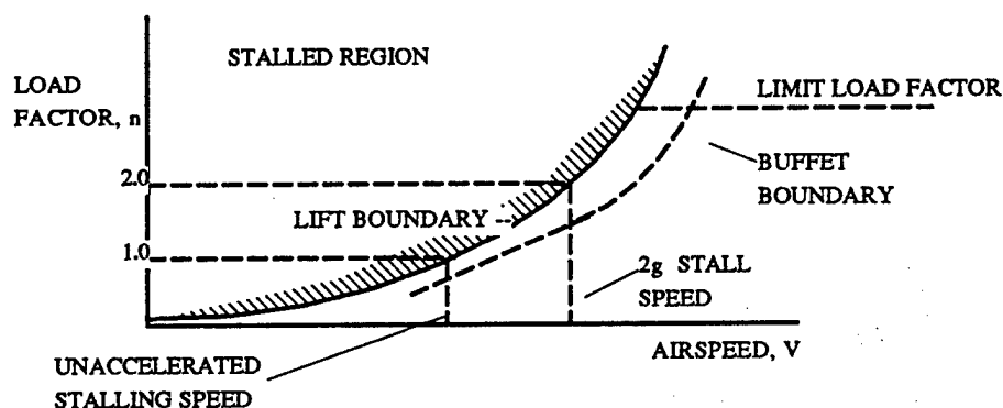
FIGURE 10.8. LOAD FACTOR EFFECTS
