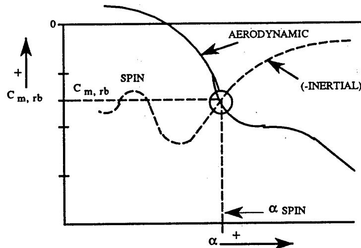
FIGURE 10.26. AERODYNAMIC PITCHING MOMENTS COMPARED TO INERTIAL PITCHING MOMENTS
