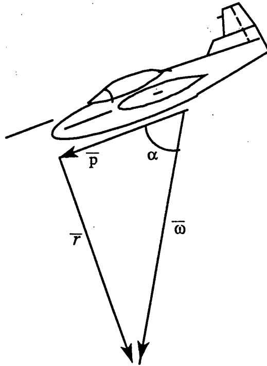
FIGURE 10.37. RESOLUTION OF SPIN VECTOR, \omega
