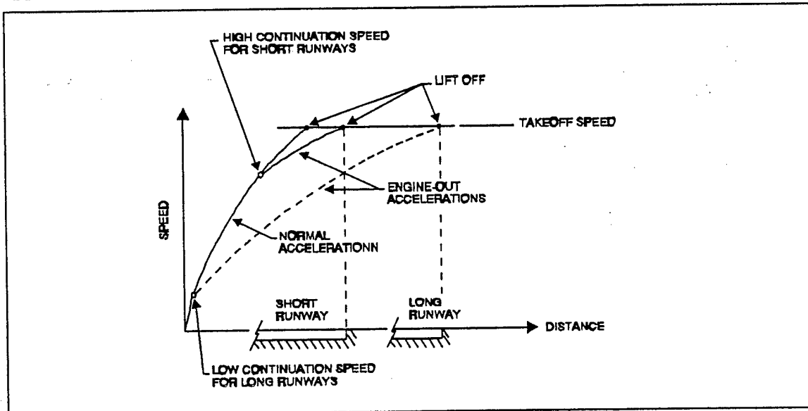
FIGURE 11.2 CONTINUATION SPEED
