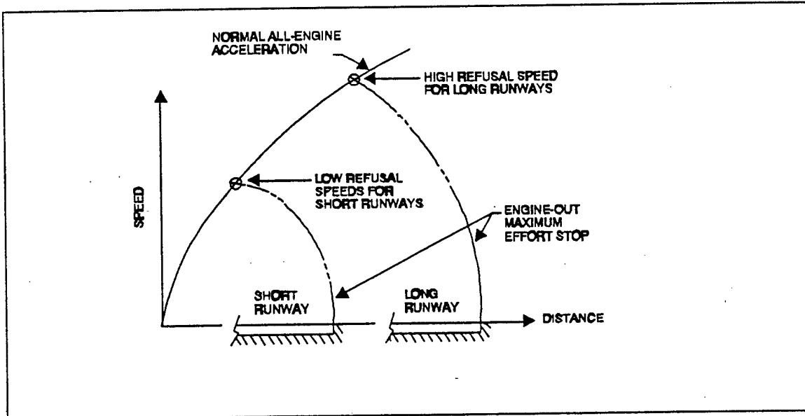
FIGURE 11.1 REFUSAL SPEED
