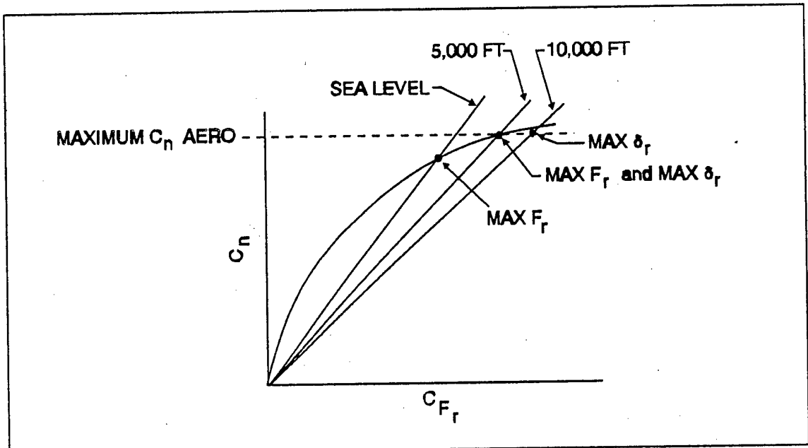
FIGURE 11.26 YAWING MOMENT LIMITED BY RUDDER FORCE
