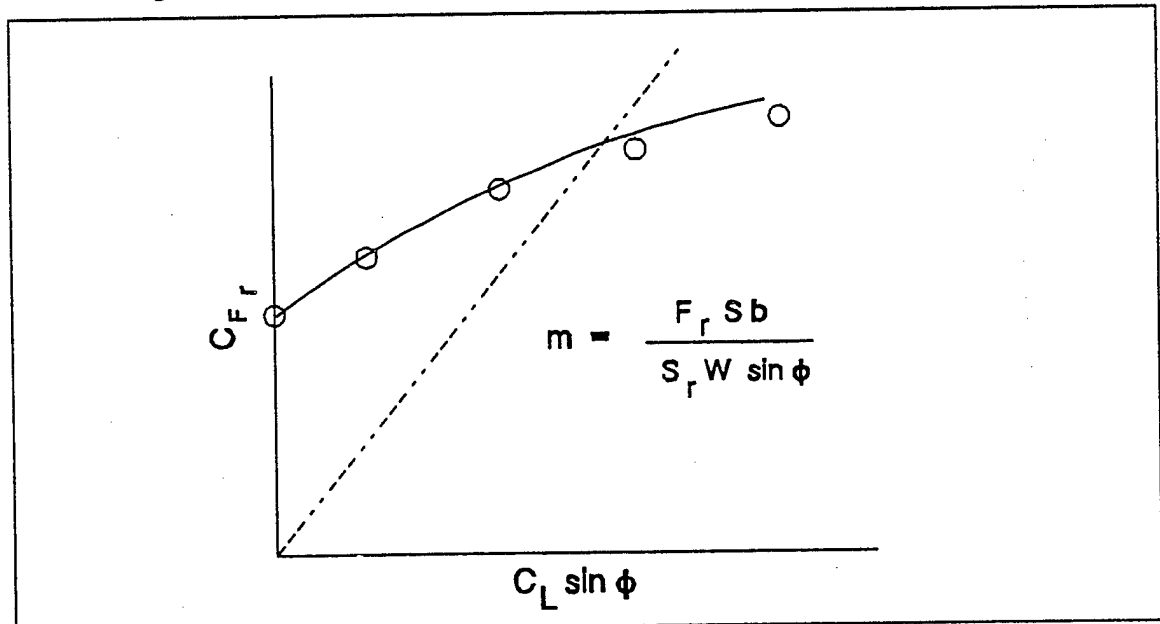
FIGURE 11.27 RUDDER FORCE COEFFICIENT VERSUS BANKED LIFT COEFFICIENT
