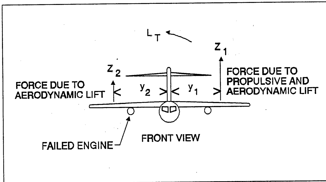
FIGURE 11.31 ROLLING MOMENTS WITH ASYMMETRIC THRUST
