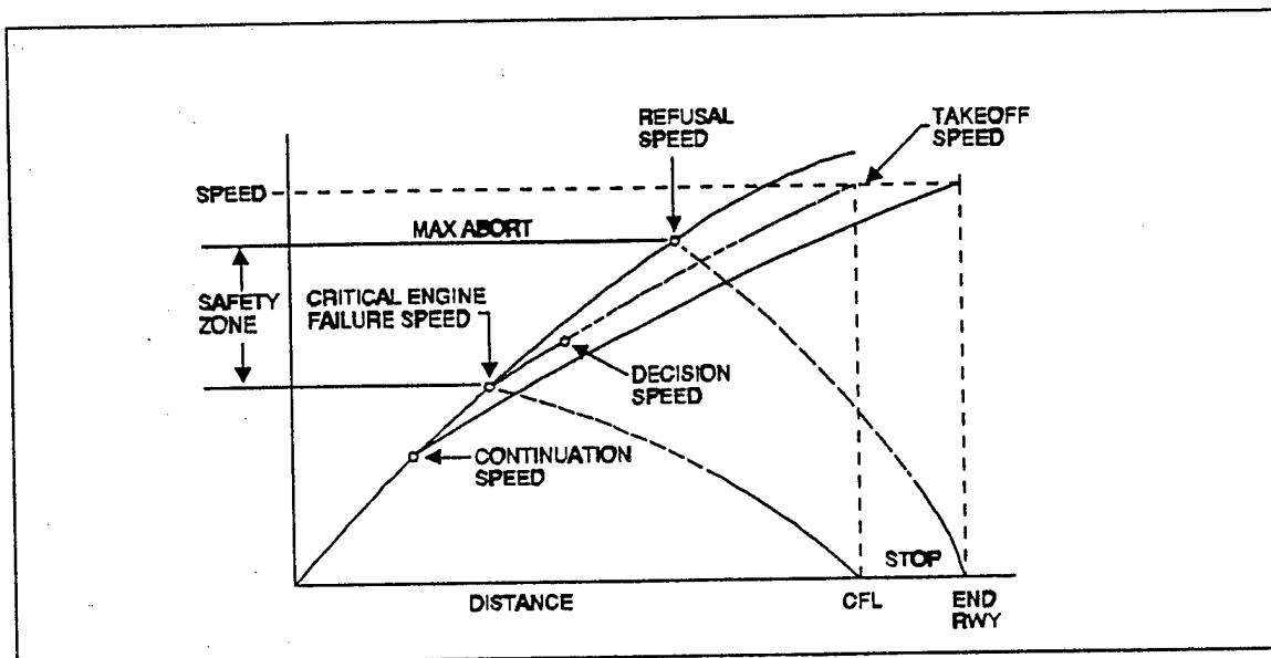
FIGURE 11.6 DECISION SPEED
