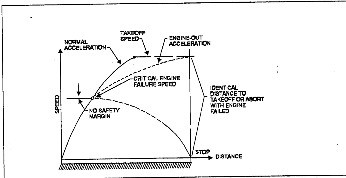
FIGURE 11.5 CRITICAL FIELD LENGTH/CRITICAL ENGINE FAILURE SPEED
