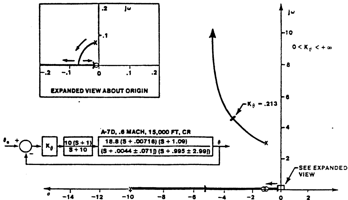
FIGURE 14.107 ROOT LOCUS OF PITCH ATTITUDE LOOP WITH LEAD COMPENSATOR
