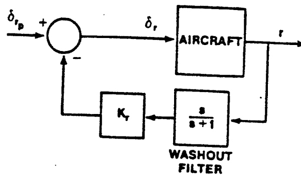
FIGURE 14.55 TYPICAL YAW DAMPER SYSTEM
