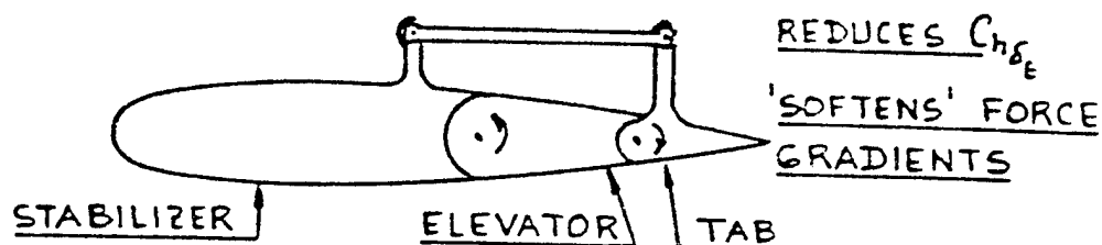
FIGURE 14.7. EXAMPLE OF LAGGING TAB
