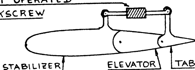
FIGURE 14.9 COMBINATION BALANCE-TRIM TAB
