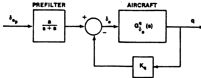
FIGURE 14.93 PREFILTER IMPLEMENTATION
