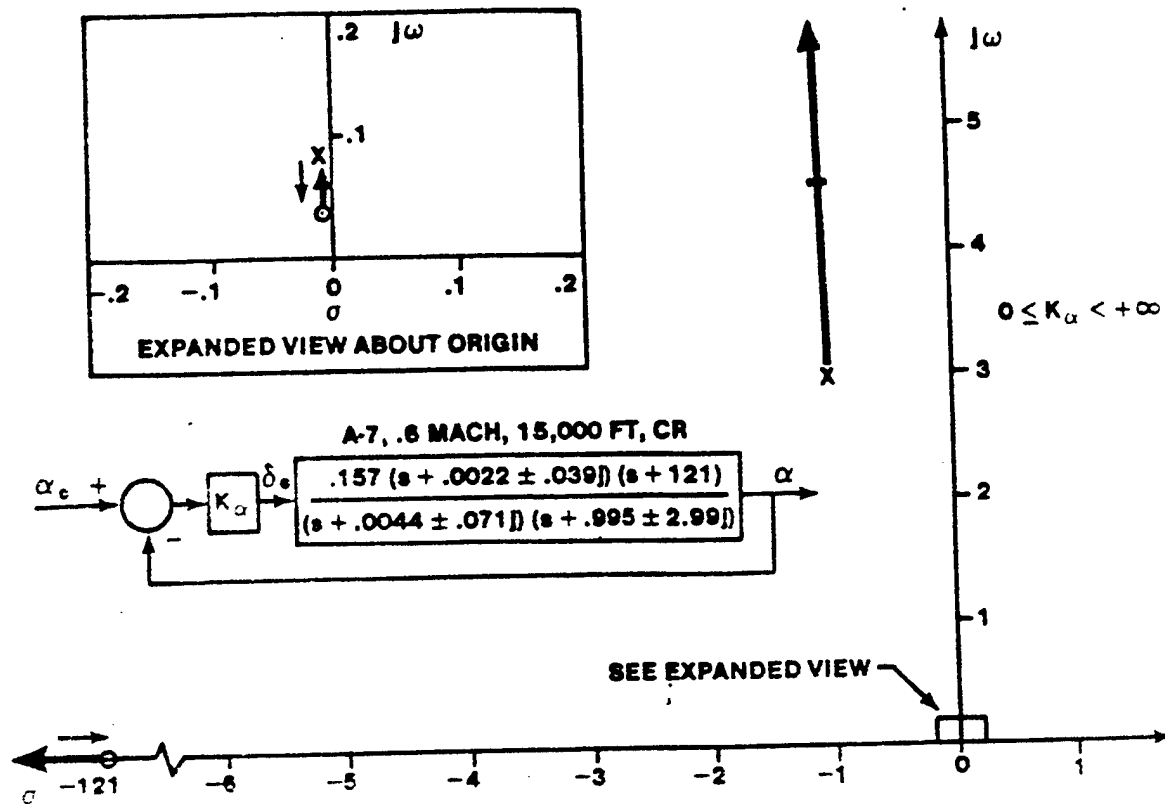
FIGURE 14.45 ROOT LOCUS PLOT OF ANGLE OF ATTACK LOOP FOR AN AIRCRAFT WITH GOOD DYNAMICS
