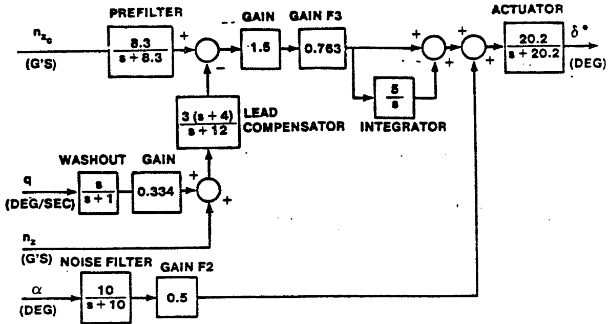
FIGURE 14.165 SIMPLIFIED F-16 LONGITUDINAL AXIS FLIGHT CONTROL SYSTEM, 0.6 MACH AT SEA LEVEL
