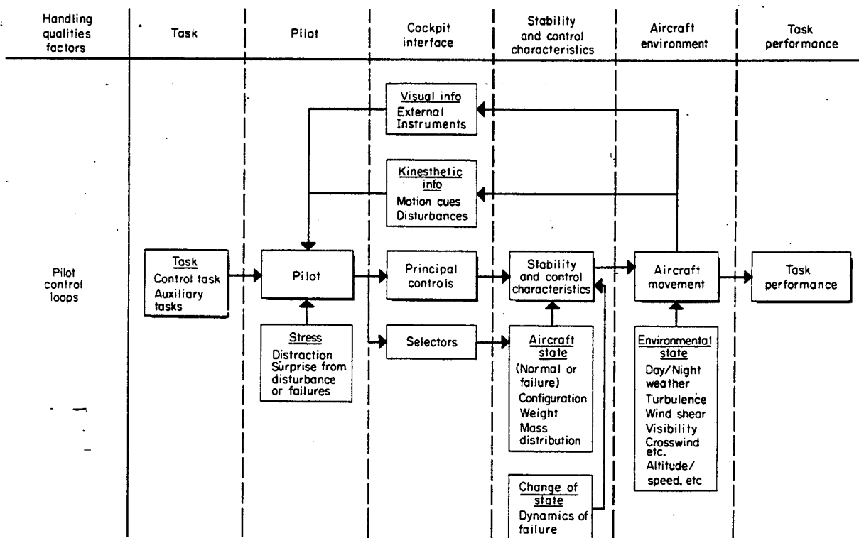
Figure 1.- Elements of control loop that influence handling qualities.
