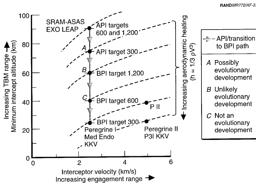
Figure 3.1—Test and Development Paths: API Transition to BPI
