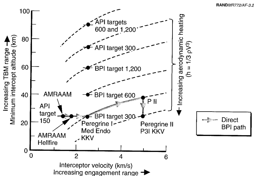
Figure 3.2—Test and Development Paths: Direct BPI Path
