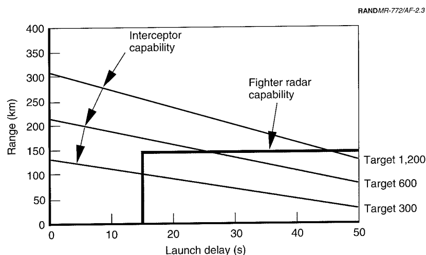
Figure 2.3—BPI Medium-Velocity Interceptor and Fighter Radar Capabilities
