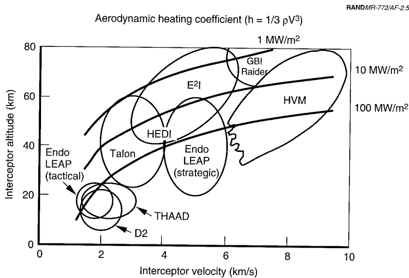
Figure 2.5—KKV Aerothermal Issues
