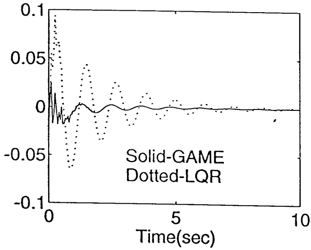
Fig. 13. Initial Response at Center
