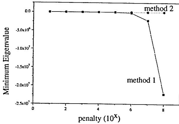
Figure (3.1.1-9) Negative Eigenvalue Magnitude as a Function of Penalty Parameter
