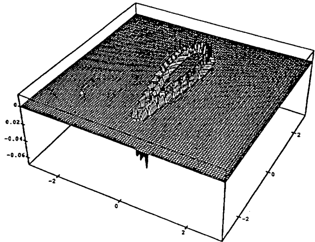
Figure (3.1.1-8) Numerical Boundary Measure for Airfoil
