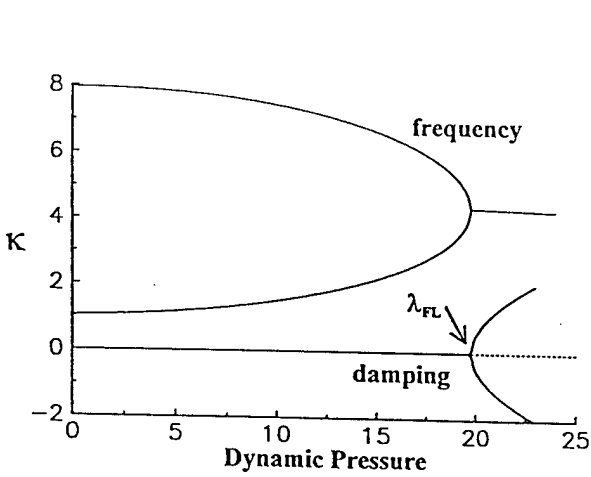
Fig. 3. The frequency and damping characteristics depend on the dynamic pressure. Flutter occurs as two (or more) modes coalesce to a common frequency and the system becomes undamped.
