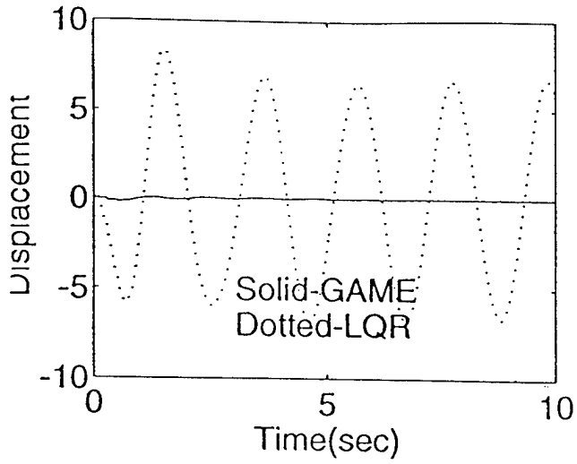
Fig. 11. Initial Response at Center
