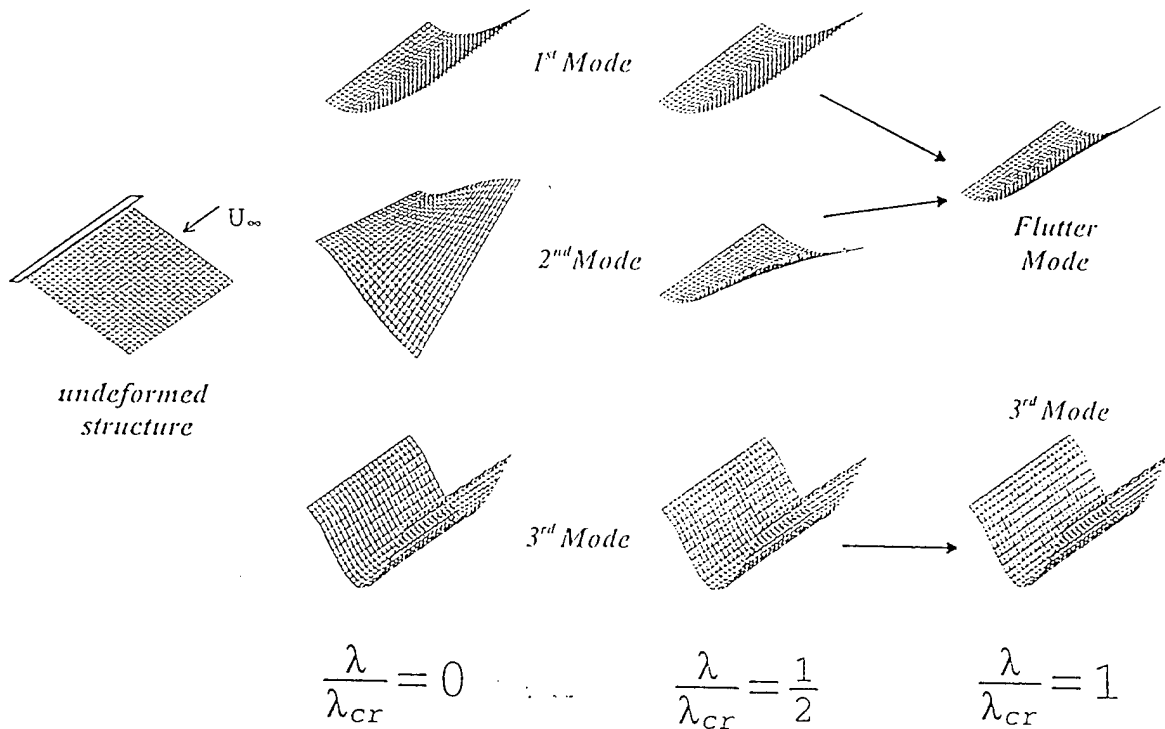
Fig. 6. The mode shapes of the cantilevered composite plate. Some modes are influenced by aerodynamic loads. The primary bending and twist mode coalesce to form the aeroelastic mode in first
