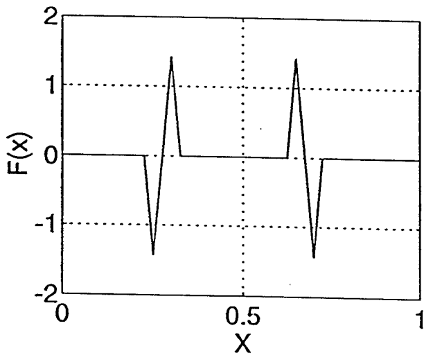
Fig. 15. Control Force
