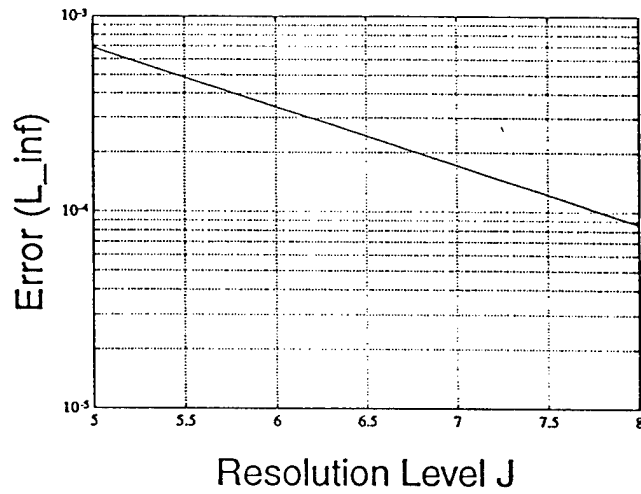
Figure (7) Asymptotic Convergence Rate, Clamped Plate 1
