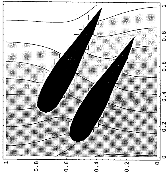
Figure (3.1.1-17) Closely Couple Airfoils, (64x64) Potential Function Contours
