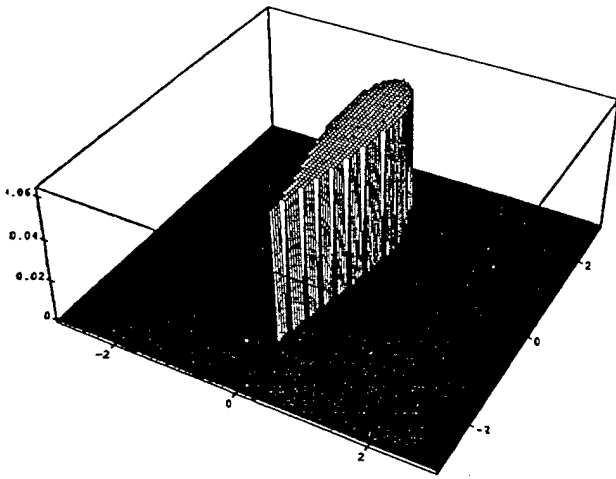
Figure (3.1.1-7) Characteristic Function of Airfoil
