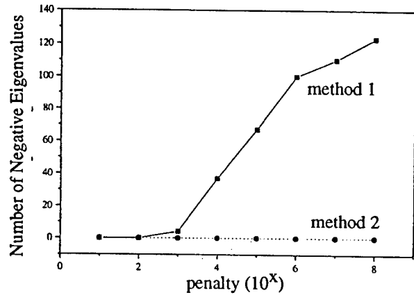
Figure (3.1.1-10) Number of Negative Eigenvalues as a Function of Penalty Parameter
