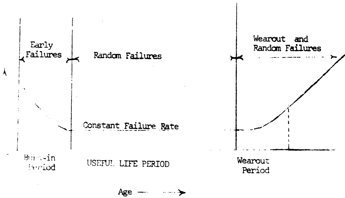
BATHTUB CURVE
