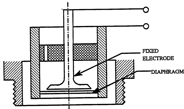
a. CAPACITIVE PRESSURE TRANSDUCER
