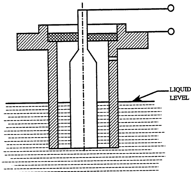
b. CAPACITIVE FUEL LEVEL TRANSDUCER
