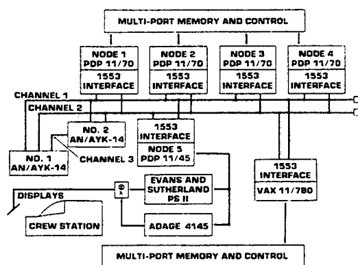
Figure 1 TASTEF Hardware Architecture
