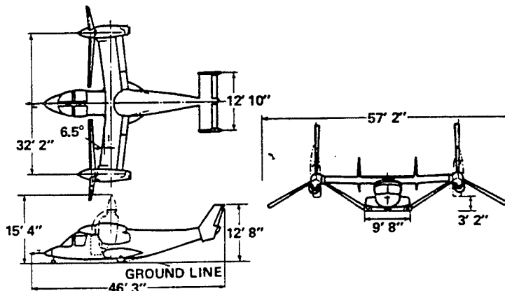
Fig. 4 XV-15 dimensions.
