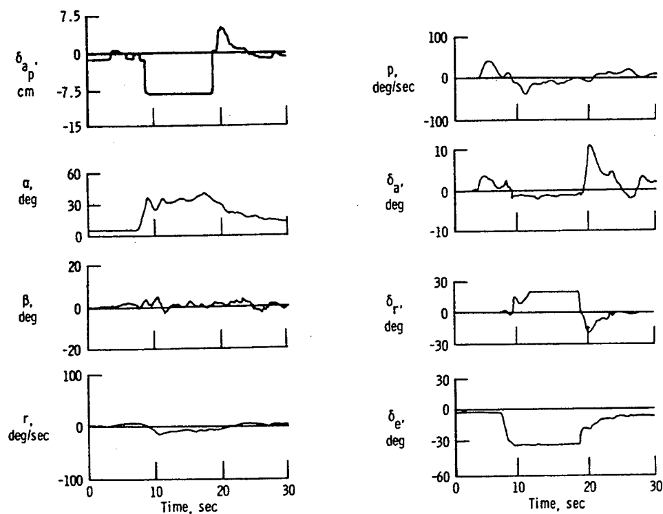
Fig. 10 The Bihrie maneuver performed by the augmented F-14. M_{\text{initial}} = 0.9 , \varphi_{\text{initial}} = 60^\circ , h_{\text{initial}} = 11,500 m.
