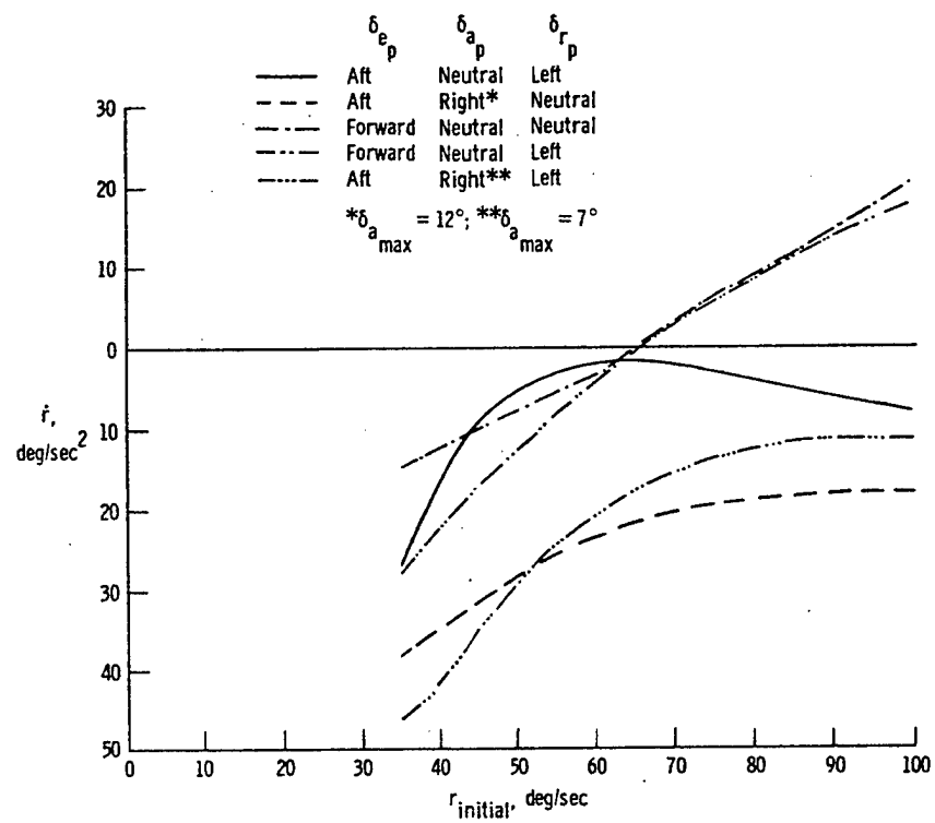
Fig. 1 Relative effectiveness of various recovery controls from an initial positive yaw rate during simulated intentional departures.
