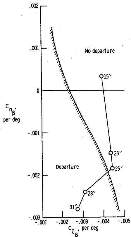
Fig. 9 The Bihrie criterion prediction of the departure susceptibility of the test airplane.
