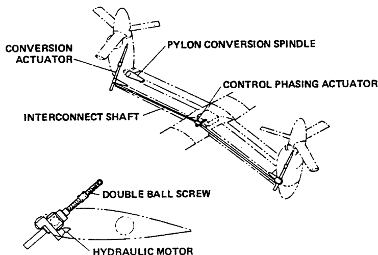
Fig. 7 Conversion system.
