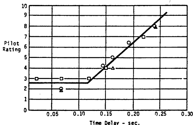
Figure 3: Effects of Time Delay On Fighter Approach And Landing Pitch Flying Quality
