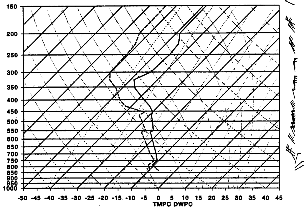
950411/1200 72489 DNR LIFT: 11 KINX: -9999 SWET: -9999 TOTL: -9999 CAPE: 0 CINS: 0 LFCV: 832 BRCH: 0
