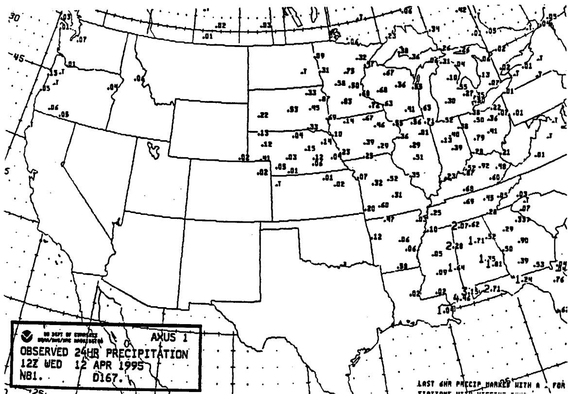
Figure 5.14 24 hr precipitation summary for 12/1200Z Apr 95
