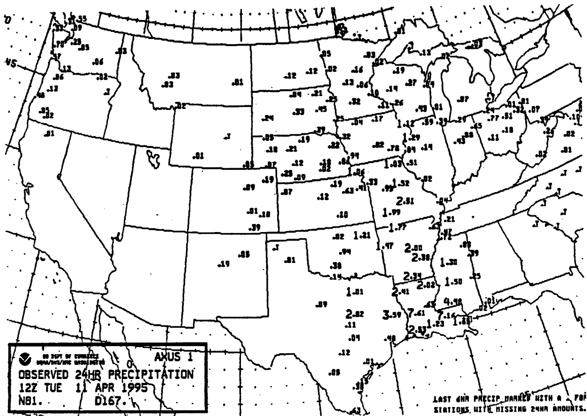
Figure 5.13 24 hr precipitation summary for 11/1200Z Apr 95
