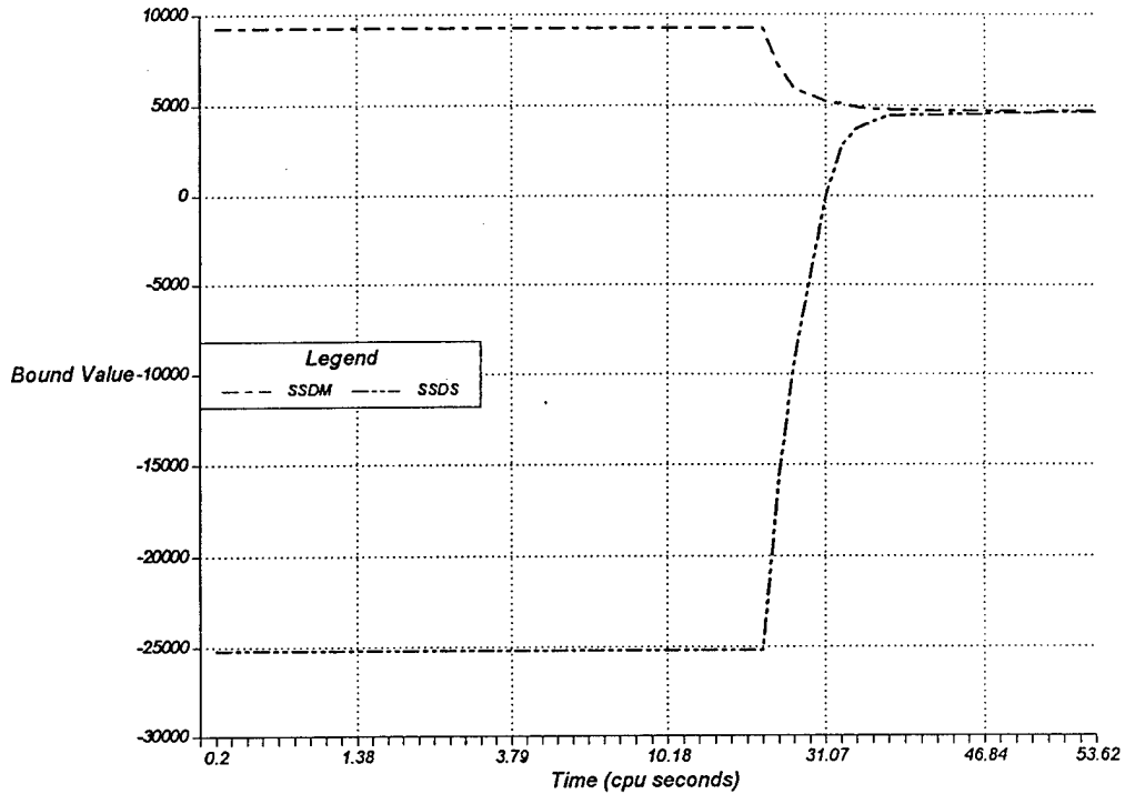
Figure 3. DW3 solves SSDM and SSDS at every iteration. These problems do not provide good bounds initially, but after thirty-five iterations without progress they begin to converge. Note that the time to solve each iteration increases markedly as the decomposition algorithm progresses. The first thirty iterations require less than half as much time as the next ten iterations. The last sixteen iterations account for over forty percent of the total solution time. SSDS determines a good upper bound after forty iterations and only improves slightly after that point. SSDM gathers cuts and improves steadily after forty iterations. DW3 halts when the objective function value of SSDM is within 0.01 of the best upper bound determined by SSDS.
