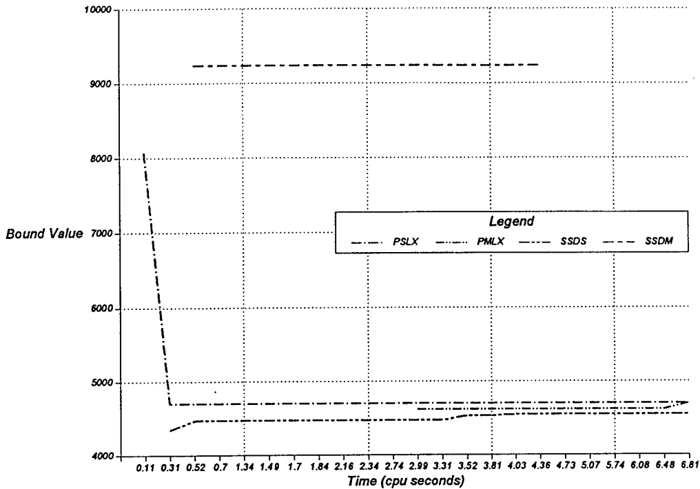
Figure 4. CD6 solves SSDS and PSLX at every iteration. These decomposition problems determine moderately good bounds initially, but do not converge rapidly. PSLX never improves the upper bound after the second iteration. When a convergence test fails, a master problem is solved. SSDM is solved more frequently than PMLX, but this problem never provides a good upper bound. PMLX provides a good lower bound when first solved on the 12th iteration. CD6 halts when the objective function value of PMLX converges with the upper bound determined by PSLX.
