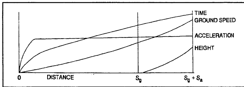
FIGURE 8.4. TAKEOFF DATA
