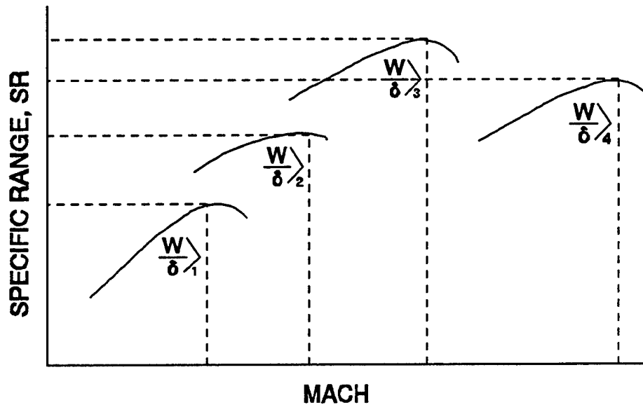
Figure 11.11 Specific Range
