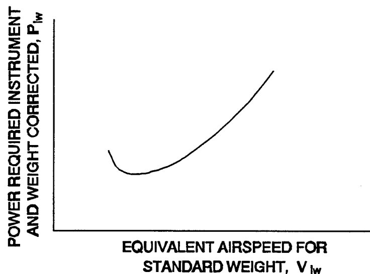
Figure 11.13 Power Required for Level Flight
