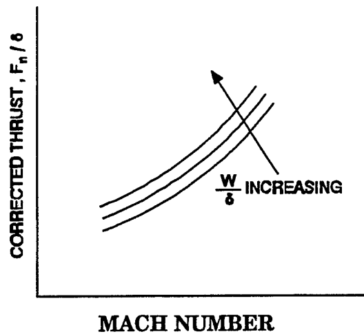
Figure 11.6 Corrected Thrust
