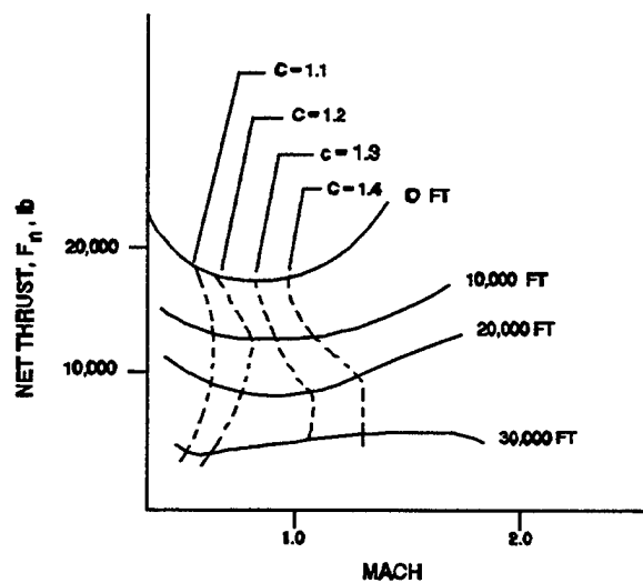
Figure 11.4 Engine Thrust Curve, 95% RPM
