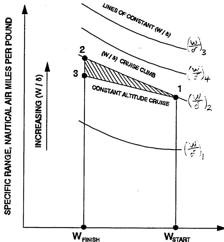
Figure 11.10 Comparison of Cruise Climb and Constant Altitude Flight
