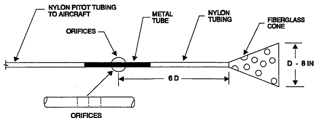
Figure 5.24 Trailing Cone Schematic
