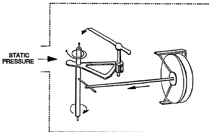
Figure 5.4 Altimeter Schematic
