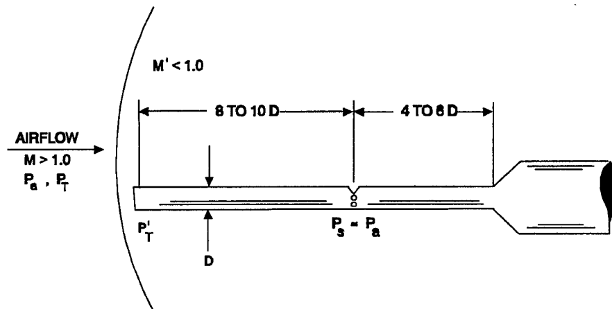
Figure 5.14 Noseboom Schematic
