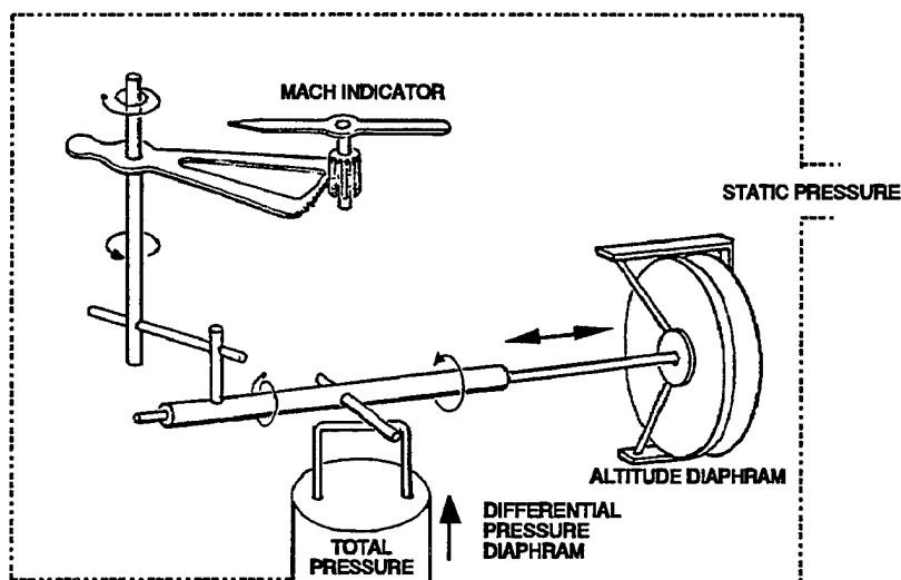
Figure 5.9 Machmeter Schematic
