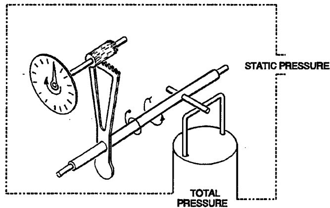
Figure 5.8 Airspeed Indicator Schematic
